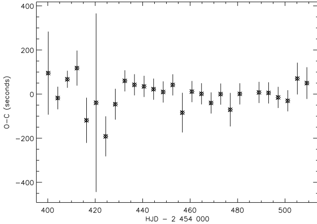
Fig. 5. The O–C diagram of the CoRoT-5b system. No clear period variation can be seen.
