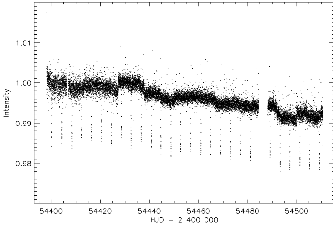
Fig. 1. Lightcurve of CoRoT-5 re-sampled to 512 s time resolution. No corrections for data jumps due to “hot pixels” have been applied in this figure to show the raw data quality.
