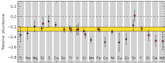
Fig. 4. Stellar abundances of CoRoT-5. Abundances found from neutral lines are marked by circles, for ionized lines box symbols are used.
