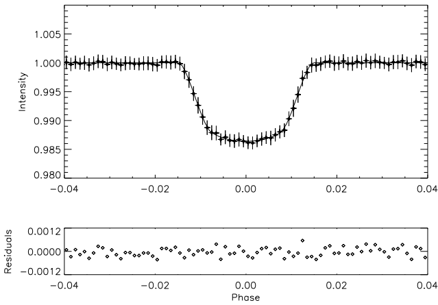
Fig. 6. Top: phase-folded lightcurve of CoRoT-5b. Bottom: residuals of fitted transit curve.
