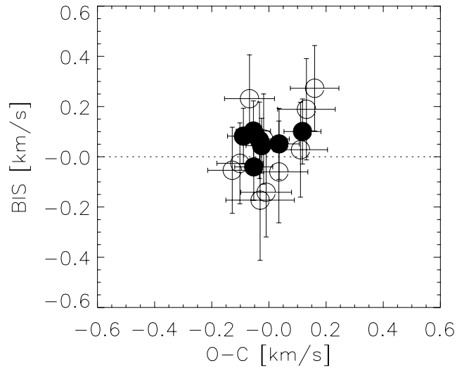
Fig. 7. Variations of the bisector span of CoRoT-17 RV data as a function of the measured velocities ( top ) and the residuals to the Keplerian fit ( bottom ). The first plot shows no correlation, a good indication for the planetary hypothesis as opposed to a blend binary signal. The second plot shows a weak correlation, owing the lowest SNR data of the sample (open points show the data where SNR is less than 5).
