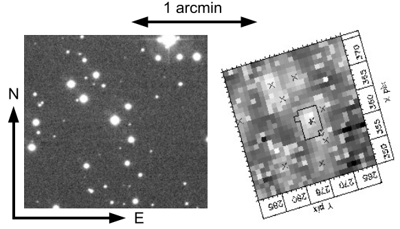
Fig. 1. Sky area around CoRoT-17 (star in the centre). Left: g -filter image with a resolution of 0.7'' taken with the CFHT telescope. Right: image taken by CoRoT at the same scale and orientation. The jagged outline in its centre is the photometric aperture mask; indicated are also CoRoT's x and y image coordinates and positions of nearby stars that are in the ExoDat database (Deleuil et al. 2009).
