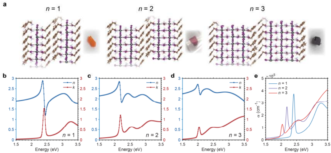
Figure 1. (a) Molecular structure of n = 1, 2, and 3 perovskites depicted with phenylethylammonium bilayers separating two QWs. Photographs of the single crystals mounted on glass substrates are shown beside each respective structure. (b – d) Optical constants and (e) absorption coefficients obtained from ellipsometry measurements for the three single crystals. The
