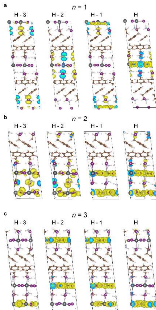
Figure 4. Wavefunction plots of the n = 1, 2, and 3 series at PBE-SOC level of theory. Wavefunctions displayed are (from left to right): HOMO-3, HOMO-2, HOMO-1 and HOMO.
