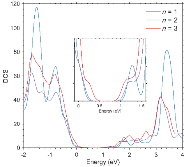
Figure 3. PBE-SOC DOS plot for the n = 1 - 3 . The inset shows the overview of the band gap region.
