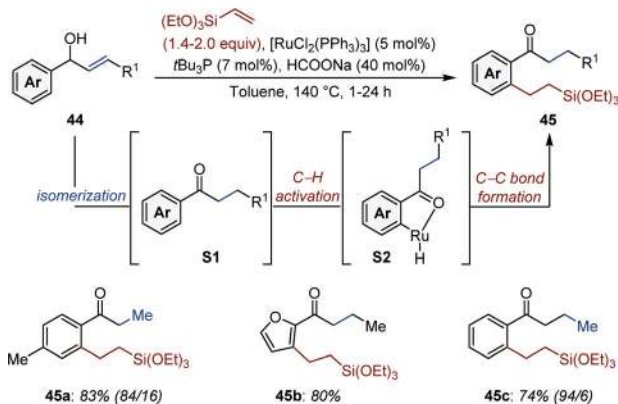
Fig. 19 Ru-Catalyzed auto-tandem isomerization/C-H activation of secondary allylic alcohols. In parenthesis is given the ratio of the products of mono- and bis-functionalization.
