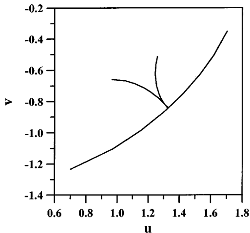
FIG. 7. Shown here is a cartoon that illustrates a difficulty that occurs in systems that do not possess time-reversal symmetry. If a system does possess time-reversal symmetry, then after a trajectory touches an equipotential it will retrace its path in coordinate space. However, in a system that does not possess time-reversal symmetry, an orbit that touches the equipotential will not retrace its path in coordinate space. The observed behavior is illustrated in this figure.
