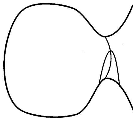
FIG. 6. Shown here is a cartoon illustrating two periodic orbits. The first orbit touches both branches of the equipotential. Orbits of this nature can be used to define transition states. The basic idea is that any trajectory that crosses this orbit from the bound region into the unbound region (that is, from the left to the right) will never return to the bound region. Thus the ionization rate can be obtained by calculating the flux across this orbit. Orbits of this nature can be found by a simple one-parameter search for periodic orbits among the orbits that initially start on an equipotential. Two types of periodic orbits are found in this manner. The first type are orbits that touch both branches of the equipotential, and the second type are orbits that touch the same equipotential twice. The transition state corresponds to an orbit of the first type. This discussion applies to systems which possess time-reversal symmetry. The system under consideration does not possess time-reversal symmetry due to the magnetic field, and thus these ideas must be modified.
