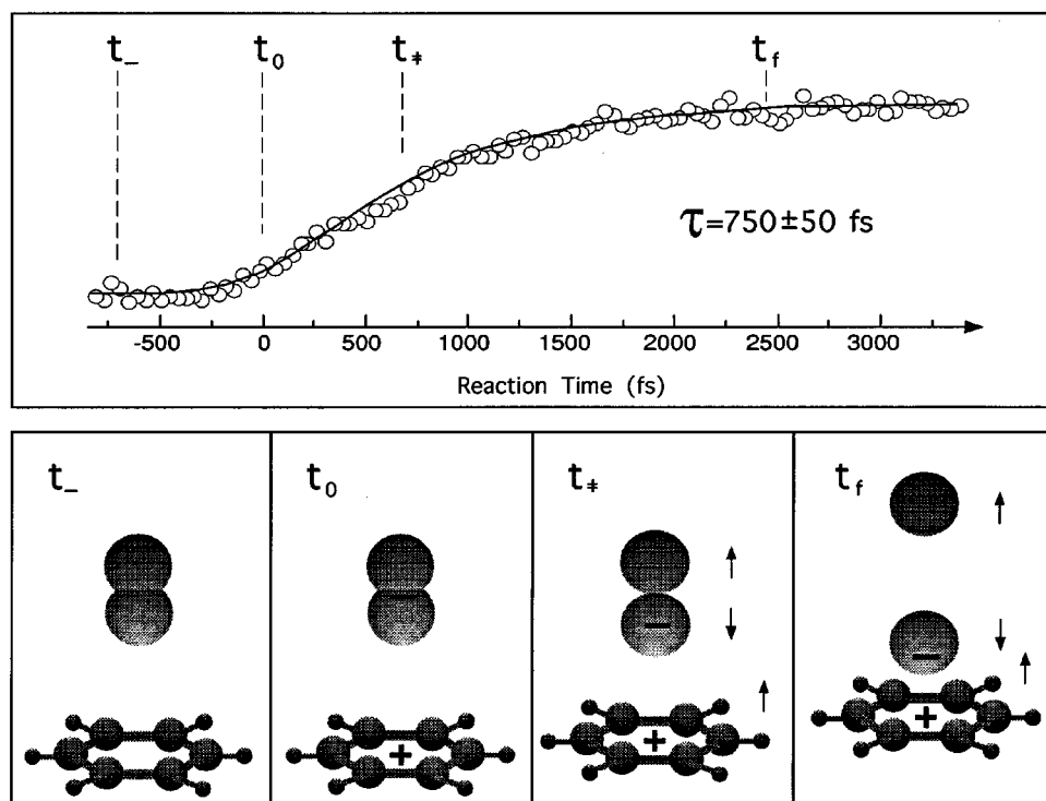
FIG. 3. fs transient of free iodine atoms (open circles) following the \text{Bz}\cdot\text{I}_2 complex excitation to its CT state by the 275 nm fs ( t=0 ) laser pulse under the 1:1 complex condition (0.5 torr Bz). A single exponential fit (solid line) to this data with a response function convolution gives a rise time of 750\pm 50 fs. We have also performed a much longer scan and found that the I atom signal stays constant for at least 200 ps for the condition of the 1:1 \text{Bz}\cdot\text{I}_2 . The four panels at the bottom describe the structural changes of the axial geometry, illustrating the complex before t=0 ( t_- ), at t=0 ( t_0 ), in the harpoon region of the PES ( t_+ ), and following the final breakage to \text{Bz}^+\cdot\text{I}^- and I products ( t_f ).
