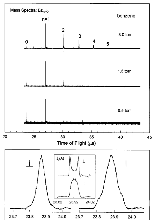
FIG. 2. Upper panel: TOF mass spectra for three benzene vapor concentrations with room temperature I_2 vapor and 800 torr of He. All spectra are normalized to the 1:1 ( Bz \cdot I_2 ) + peak for clarity. Note that these ions are produced by a 1+1 REMPI process, as all clusters have strong CT absorption in this wavelength region and the two-photon energy ( \sim 9.0 \text{ eV} ) lies just above their ionization potentials. Therefore, the size distribution should closely reflect the true beam composition, and this is further supported by the temporal response described in the text. Lower panel: Iodine-atom TOF distributions for two pump-laser polarizations, perpendicular (left) and parallel (right) to the TOF axis (the TOF times are different in the two panels because of the acceleration voltages). For comparison, the insert shows TOF distributions of I_2(A) state (at 690 nm) through its perpendicularly polarized X \rightarrow A transition; the splitting gives \sim 850 \text{ cm}^{-1} of translational energy for the I atom.
