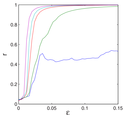
FIG. 3. (Color online) The global order parameter versus the coupling parameter for p_o=0.001, 0.01, 0.05, 0.1 , and 0.2 , corresponding to the curves from bottom up. For very small p_o , only clustering occurs. Global synchronization can be achieved with increase of p_o . The network parameters are N=500, M=5 , and p_i=0.7 .
