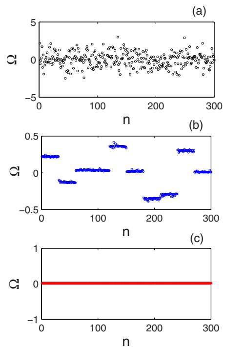
FIG. 2. (Color online) For a clustered network of N=300, M=10, p_i=0.7 , and p_o=0.002 , (a)–(c) final frequency distribution for \epsilon=0.01, 0.5 , and 1.0 , respectively. Global synchronization has already occurred for \epsilon=1.0 .
