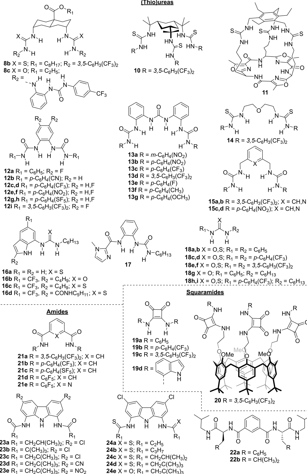
Figure 5. Small neutral molecules with acidic NH groups reported as HCO 3 - transporters after 2011.
