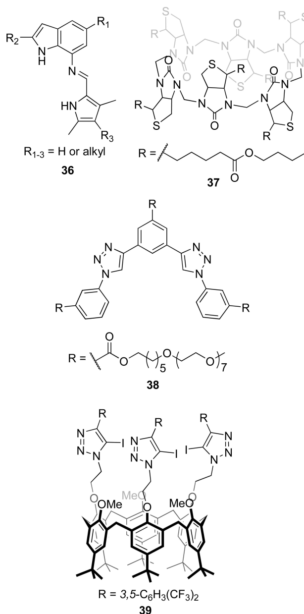
Figure 9. Efficient \text{Cl}^- transporters that showed no activity as \text{HCO}_3^- transporters.
