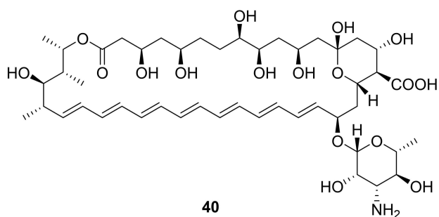
Figure 12. Natural HCO 3 - transporter Amphotericin B.
