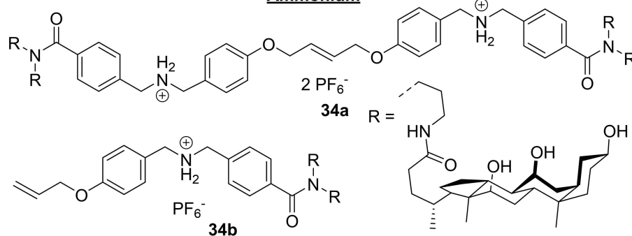
Figure 6. Cationic molecules reported as HCO_3^- transporters after 2011.
