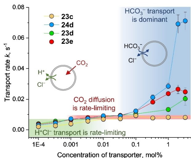
Figure 11. Rate constants as measured in the Eu1 assay for \text{HCO}_3^- transport for different concentrations of carbazole-based transporters, showing that different mechanisms dominate at different stages. Reproduced from Ref. [72] with permission from the Royal Society of Chemistry.
