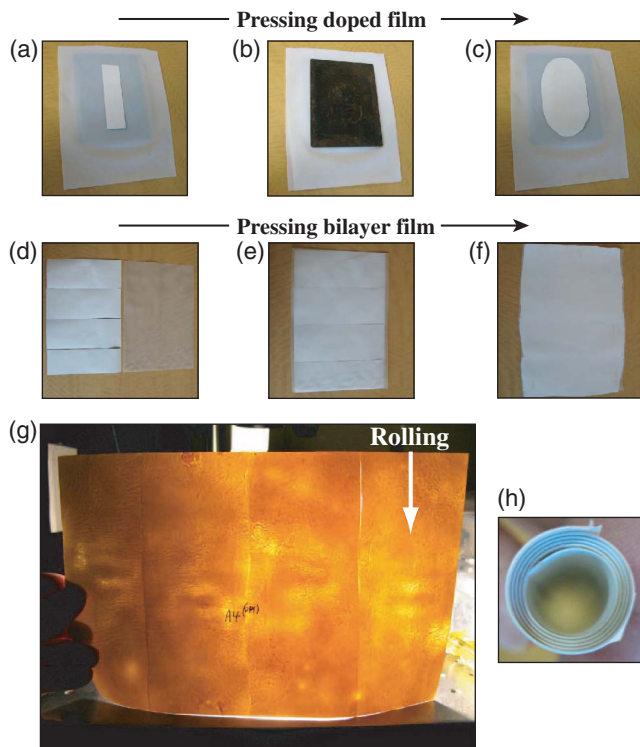
Fig. 3. (Color online) Fabrication steps of a \text{TiO}_2 -doped polymer Bragg fiber. (a)–(c) Strips of \text{TiO}_2 film ( \sim 400 \mu\text{m} thick) are pressed to a thinner thickness ( \sim 100 \mu\text{m} ). (d)–(f) High- and low-index films are pressed together to form a bilayer. (g) defects in the bilayer. (h) Bilayer is rolled into a Bragg fiber.
