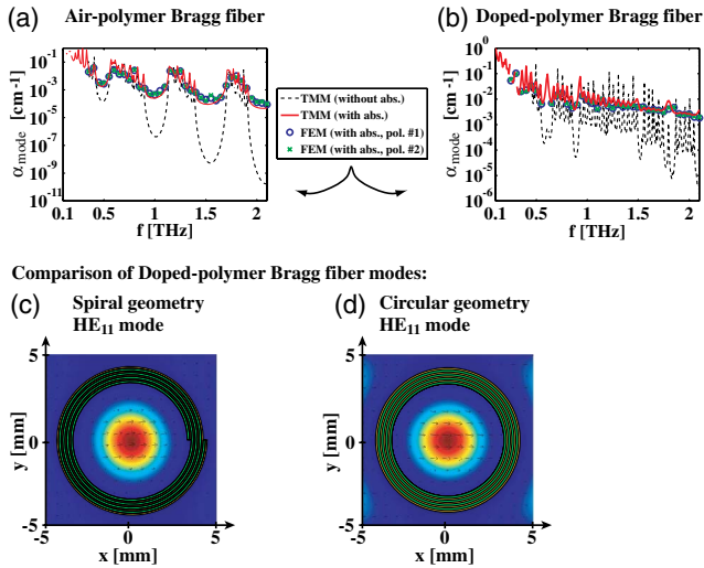
Fig. 5. (Color online) Comparison of the theoretical HE_{11} mode propagation losses of a doped-polymer Bragg fiber with ideal (circular) and nonideal (spiral) geometry. The propagation losses in the case of the circular geometry are calculated using a transfer matrix method (TMM). The solid and dashed lines, respectively, correspond to simulations with and without material absorption. The propagation losses in the spiral geometry (circles and crosses) were calculated with a finite element method (FEM) mode solver. The dimensions and material parameters are described in the text. (a) Air-polymer Bragg fiber, (b) doped-polymer Bragg fiber. There is good agreement between the results indicating that the spiral defect does not significantly effect fiber losses. The similarities are further illustrated by comparing the power distribution and electric field orientation of the HE_{11} mode in the spiral (c) and circular (d) geometries. The modes are seen to be nearly identical.
