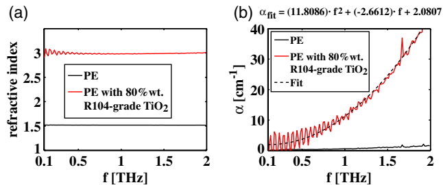
Fig. 2. (Color online) THz refractive index (a) and power absorption loss (b) of pure and \text{TiO}_2 -doped polyethylene films. Fabry-Perot oscillations due to the thickness of the samples can be seen. Absorption loss from the doped film can be approximated by a quadratic function.
