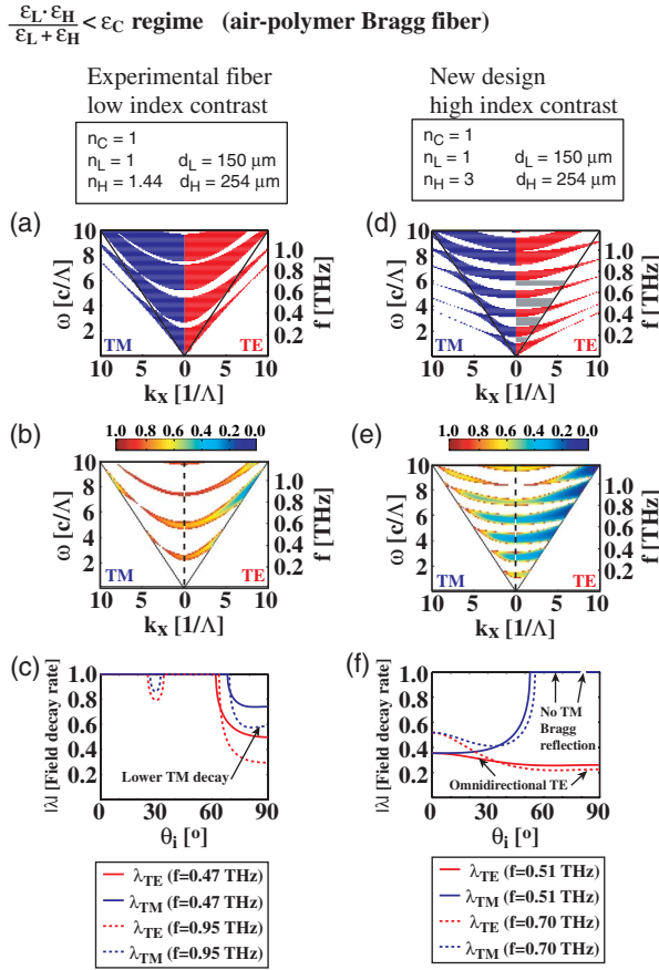
Fig. 11. (Color online) Band diagrams and field decay rates of air-polymer planar Bragg reflectors where \epsilon_L = \epsilon_C \left( \frac{\epsilon_L \epsilon_H}{\epsilon_L + \epsilon_H} < \epsilon_C \right) . First column uses parameters of experimental Bragg fiber, second column considers a 25 vol.% Cu-doped PE Bragg fiber. First row presents the band diagram of the reflectors. Second row presents \lambda diagrams of the field decay rates within the bandgap regions. Third row presents cuts of the \lambda diagrams at constant frequencies.
