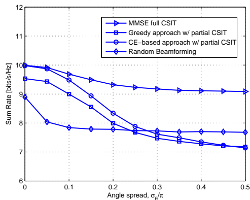
Figure 3: Sum rate as a function of angle spread for various user selection schemes with N_t = 2 , antenna spacing d = 0.5\lambda and K = 50 users.
