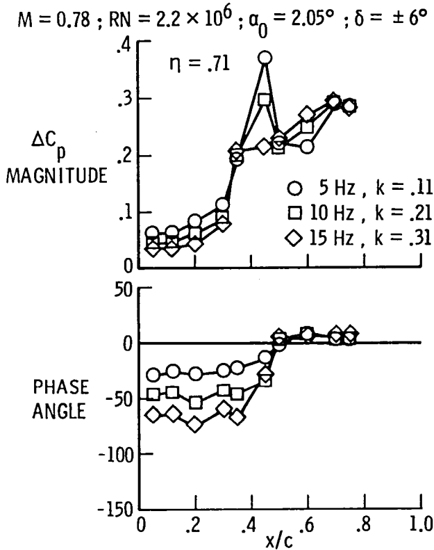
Fig. 10.- Outboard control surface oscillating frequency results.
