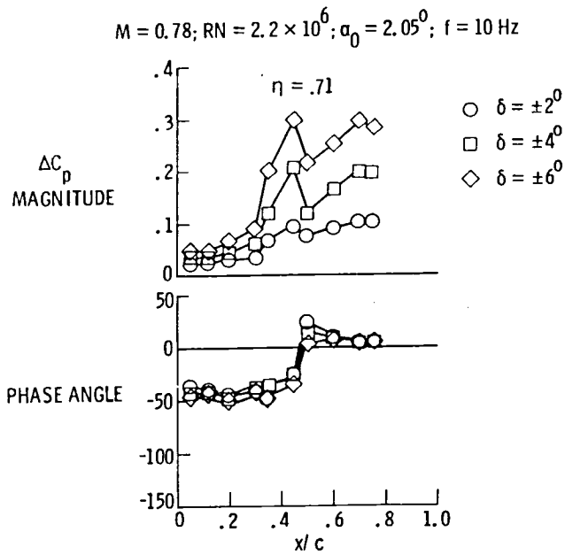
Fig. 9.- Outboard control surface oscillating deflection results.
