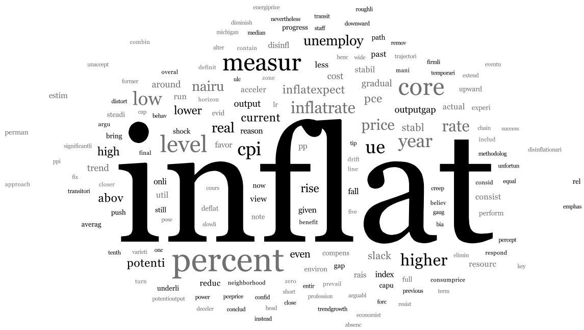
Figure 2: Topic 25—“Inflation”
