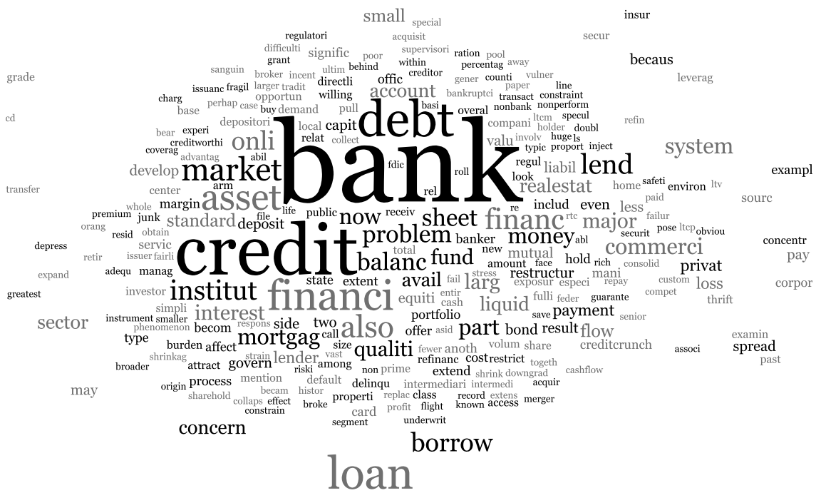
Figure 3: Topic 38—“Banking”
