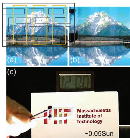
FIG. 4. (Color) (a) Picture of the “Teton mountains” displayed on a LCD screen (b) with the fully assembled transparent solar cell in front of the picture. In (a) the anode/active layer drawing is overlaid on the same picture and the orange boxes highlight the active layer area. (a) and (b) were taken side-by-side during the same exposure. (c) Picture of the series-integrated, transparent cell illuminated with \sim 0.05 sun while allowing for high transparency. See Ref. 12.
