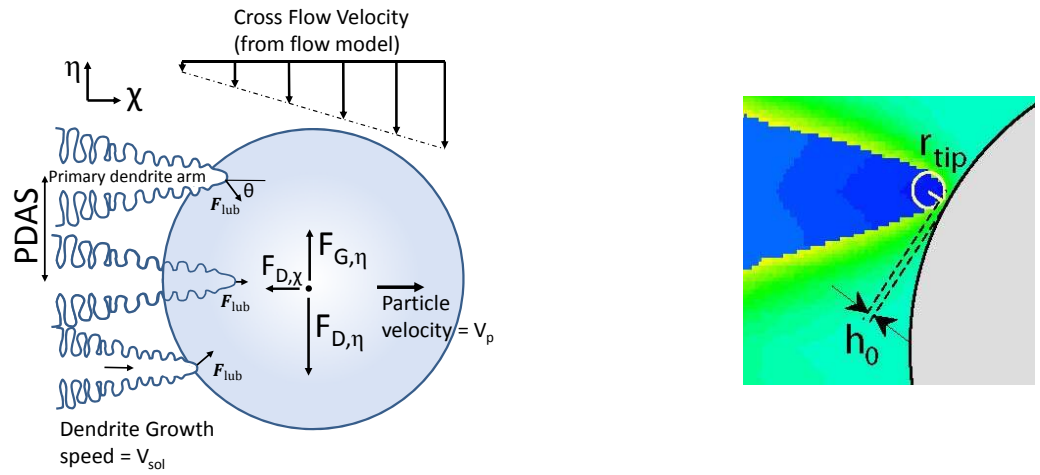
(a) Particle touching three dendrite tips
