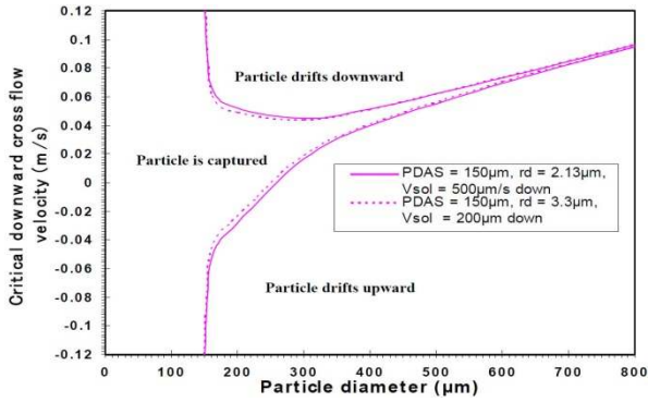
(c) Effect of Solidification Front Velocity, (Argon Bubbles)
