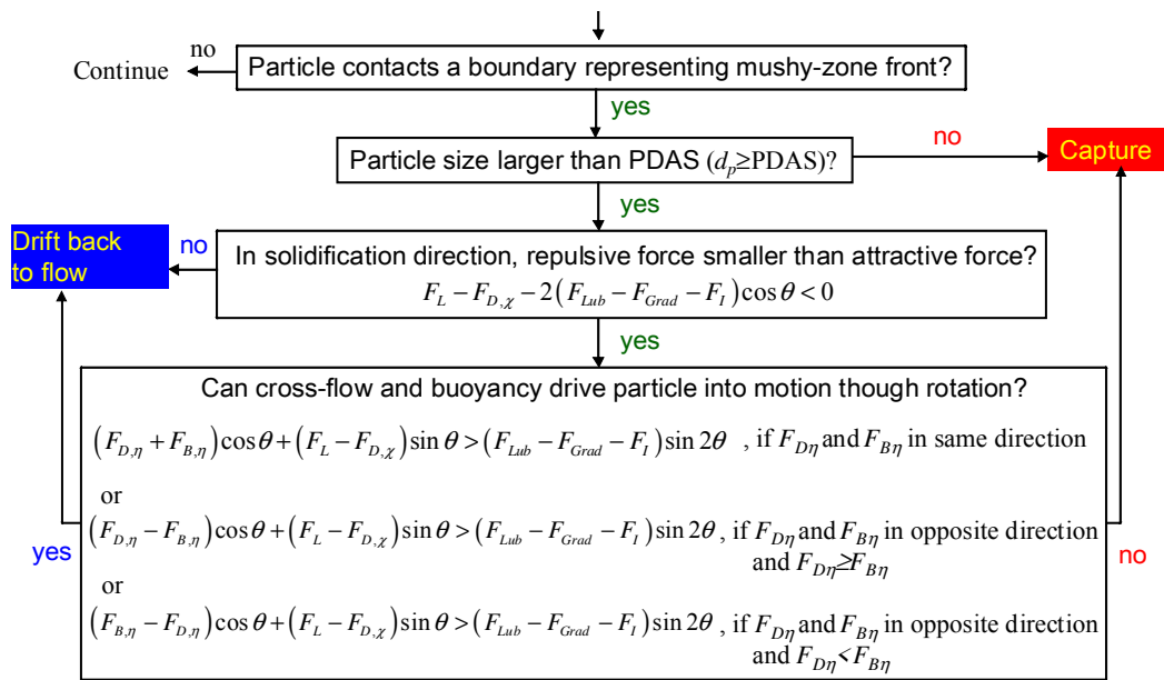
Figure 4. Flow chart for the shell entrapment criterion
