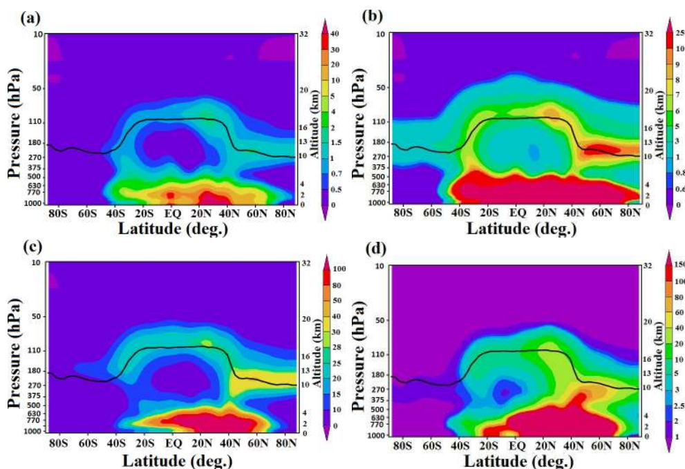
Fig. 3. “cross section” (averaged for June–September and 60\text{--}120^\circ\text{E} ) of concentrations ( \text{ng m}^{-3} ) of (a) BC aerosols, (b) OC aerosols, (c) \text{SO}_4^{2-} aerosols, and (d) mineral dust aerosols. The black line marks the longitudinally averaged tropopause showing increased height in the ASM region.
