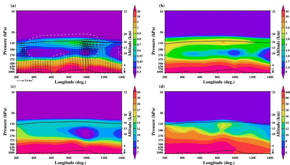
Fig. 2. “cross section” (averaged for June–September and 15\text{--}35^\circ\text{N} ) of concentrations ( \text{ng m}^{-3} ) of (a) BC aerosols, location of the monsoon anticyclone indicated with dotted line, (b) OC aerosols, (c) \text{SO}_4^{2-} , and (d) mineral dust aerosols. Vectors of the circulation are shown in (a) with the vertical wind scaled by 300. The upper black line marks the latitudinally averaged tropopause showing increased height in the ASM region. The lower black line marks the topography. The dashed white line is the negative 10^{-5} vorticity contour showing the approximate region of the anticyclone.
