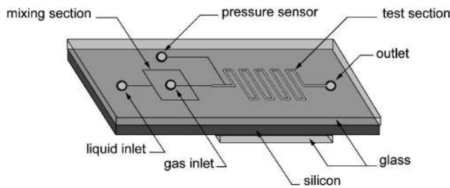
FIG. 1. Two-phase flow microchannel module: mixing section ( 50\ \mu\text{m} square channel), test section ( 200 or 525\ \mu\text{m} square channel).
