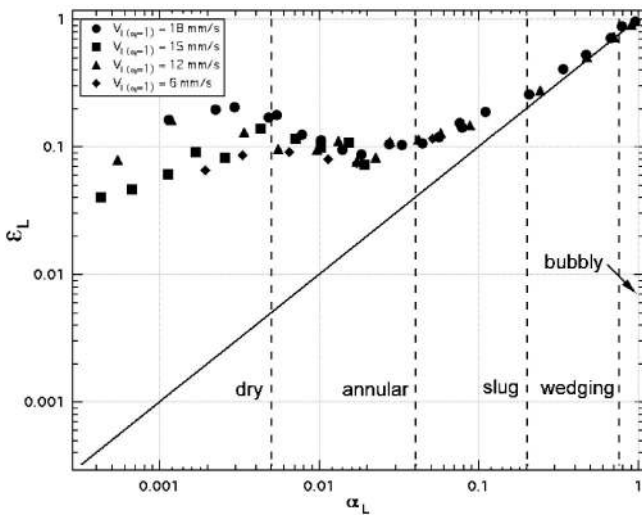
FIG. 8. Apparent liquid fraction \epsilon_L vs homogeneous liquid fraction \alpha_L for different initial conditions ( h=525 \mu\text{m} ).
