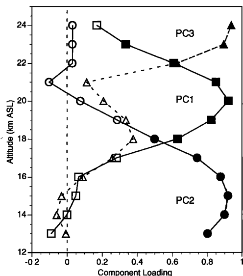
Figure 3. Loadings (correlation coefficients) from the orthogonal varimax transformation of the three significant principal components plotted as a function of altitude. Solid symbols represent those loadings considered statistically significant.
