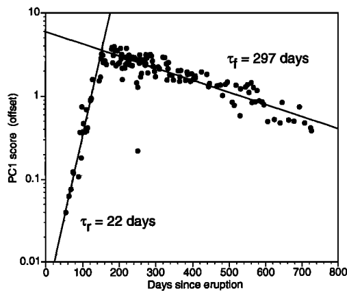
Figure 6. Principal component scores for PC1 with exponential least squares fit of the rise and fall portions of the curve. The 1/e time constants for the rise and fall are 22 and 297 days, respectively.
