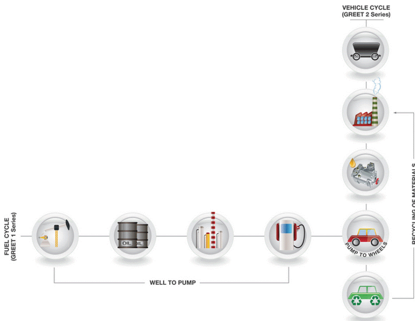
Figure 11.1. GREET Model
