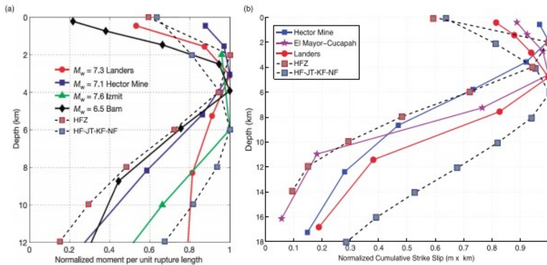
Figure 8. Distributions of coseismic slip for several \sim M7 strike-slip earthquake integrals along the rupture length, normalized by their max value as a function of depth (Fialko et al., 2005) together with the Humps fault zone and Hope-Jordan Thrust-Kekerengu-Needles fault segments. The figure is modified after (a) Fialko et al. (2005) and (b) X. Xu et al. (2016), respectively.
