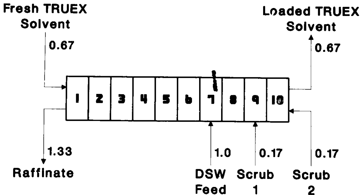
Fig. B-1. The Experimental Design and Flow Ratios of the Two Countercurrent Experiments (Boxes numbered 1-10 represent the separatory funnels or stages)
