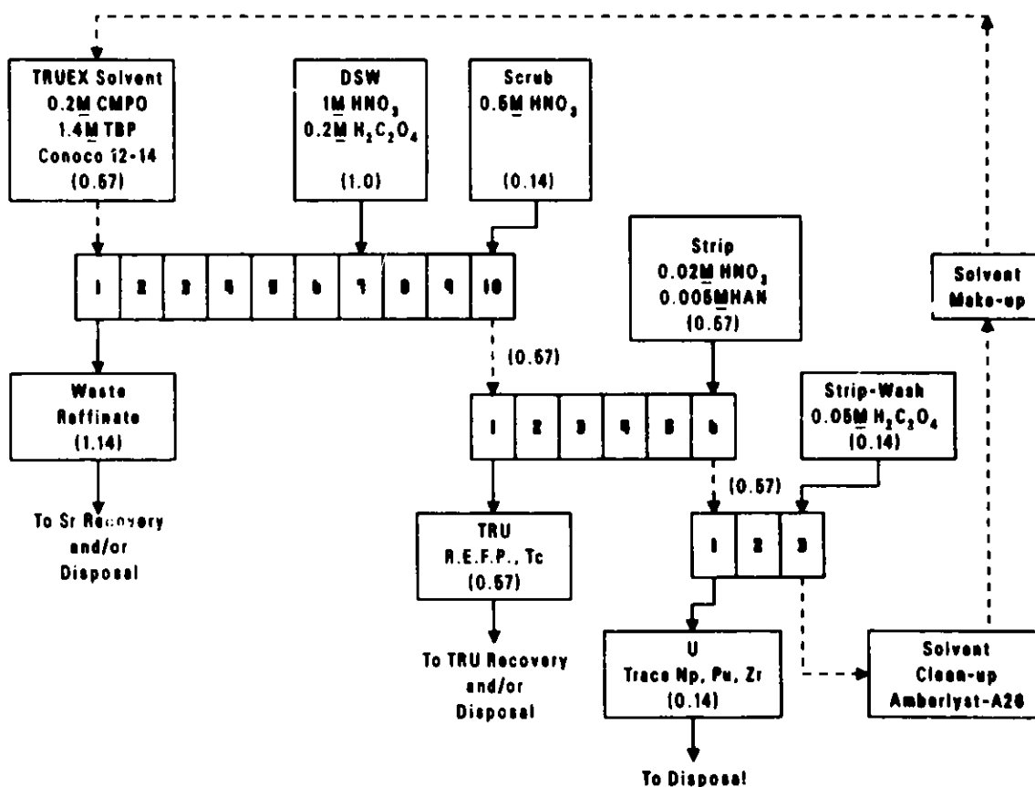
Fig. IV-11. An Improved CMPO-TRUEX Flowsheet for DSW Feed. (The number in parentheses in each box is the relative flow rate of that stream.)
