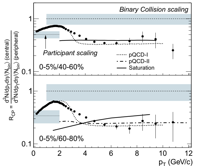
FIG. 4: R_{CP}(p_T) vs. p_T for (h^+ + h^-)/2 . Error bars include both statistical and systematic uncertainties. Calculations are described in the text.
