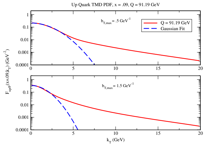
FIG. 3 (color online). Comparison of the TMD PDF at Q = 91.19 GeV with a Gaussian fit for the two different values of b_{\max} = 0.5, 1.5 \text{ GeV}^{-1} . (See online version for color.)
