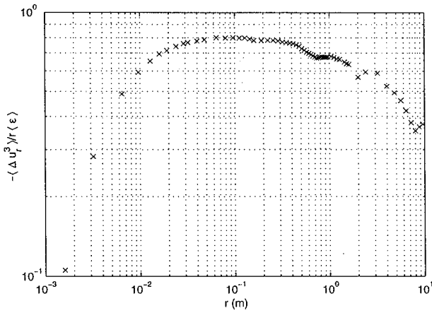
FIG. 1. Normalized third-order structure function, S_3 \equiv \langle \Delta u_r^3 \rangle / r \langle \varepsilon \rangle , where \varepsilon = 15\nu \langle (\partial u / \partial x)^2 \rangle , plotted against the separation distance r . A scaling range of more than a decade is likely. The magnitude of S_3 is not far from 0.8 in the region where it is roughly flat, as expected from Kolmogorov's four-fifths law; it is both interesting and nontrivial that the law appears to hold quantitatively even in inhomogeneous turbulence. First and second sets of data from Table I have been combined.
