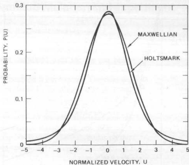
FIG. 4. One-dimensional Maxwellian and Holtzmark velocity distributions for \sigma^2 = 2 .
