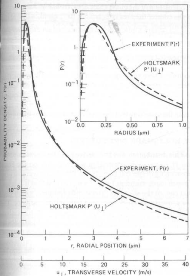
Fig. 2. Probability density function for target current density in single-lens column fitted with a Holtzmark distribution.
