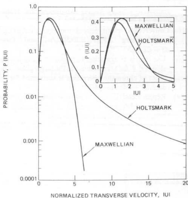
FIG. 5. Two-dimensional Maxwellian and Holtzmark distributions for \sigma^2 = 2 .
