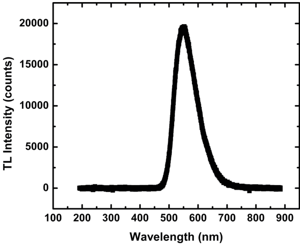
Figure 9. TL emission spectrum at 262°C for Ce:YAG 0.14%.
