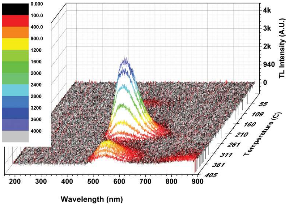
Figure 7. TL intensity versus temperature and wavelength.
