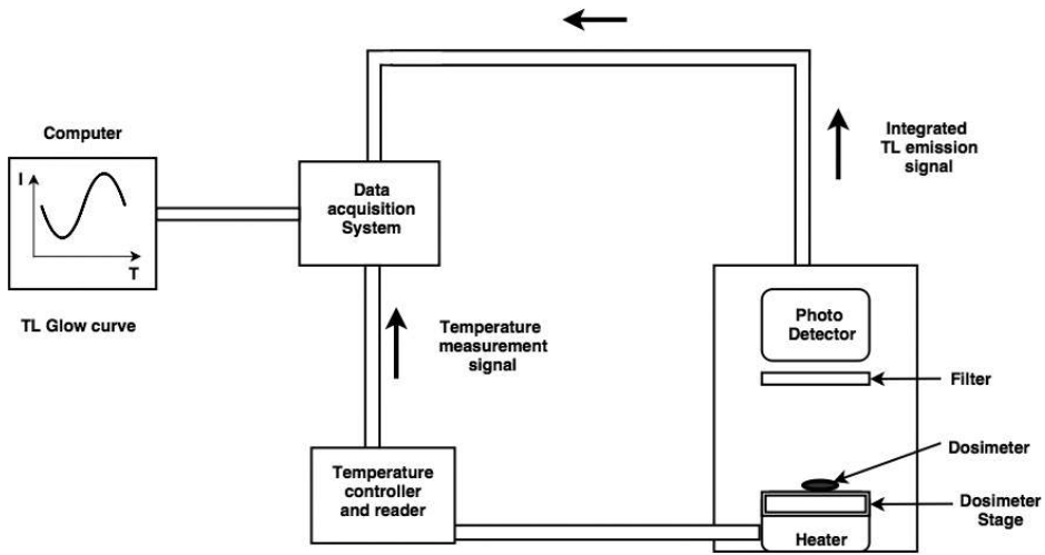
Figure 5. Schematic of TLD reader setup [73].
