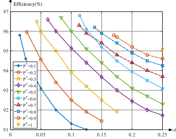
Fig. 9. The simulation results of efficiency with different powers and phase shifts.
