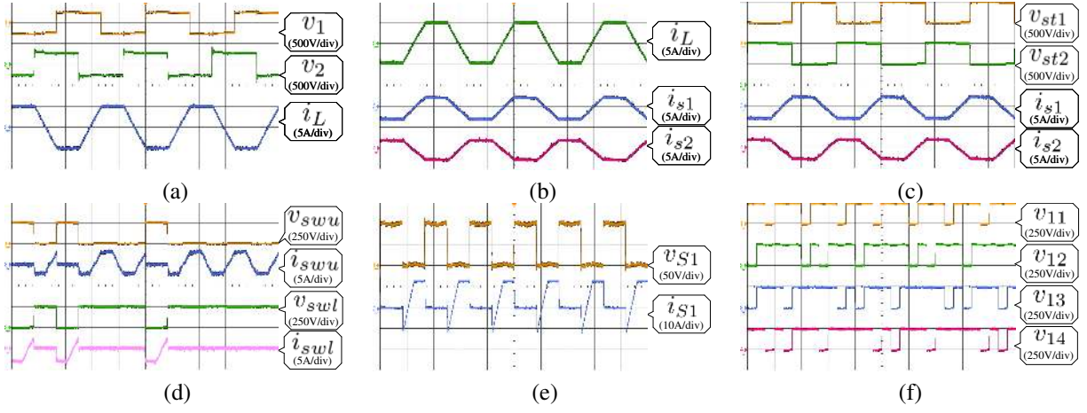
Fig. 13. Experimental waveforms of reverse power flow with P^* = -1 . (X-axis: Time, 100 \mu\text{s}/\text{div} ): (a) voltage and current of inductor; (b) current sharing performance between two stacks; (c) voltages and currents of stacks. (X-axis: Time, 200 \mu\text{s}/\text{div} ): (d) voltages and currents of upper switch ( v_{swu} and i_{swu} ) and lower switch ( v_{swl} and i_{swl} ) in SMs; (e) voltage and current of the switch S_1 in active bridge. (X-axis: Time, 500 \mu\text{s}/\text{div} ): (f) SM output voltages.
