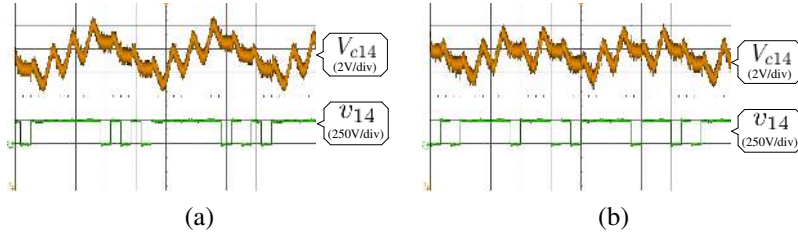
Fig. 14. Experimental waveforms of SM capacitor voltage and SM output voltage (X-axis: Time, 500 \mu\text{s}/\text{div} ). (a) Large voltage ripple modulation. (b) Small voltage ripple modulation.
