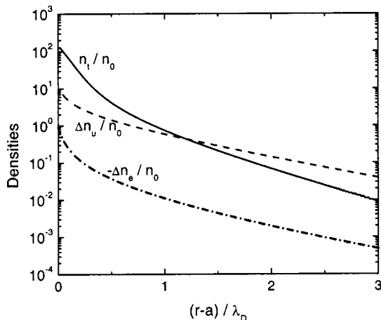
FIG. 2. Trapped ion density [ n_t(r) , solid], deviation of untrapped ion density from ambient [ \Delta n_u(r) , dashed], and deviation of electron density from ambient [ -\Delta n_e(r) , dotted–dashed], all scaled to ambient density n_0 , for Case 1: T/T_e = 0.01 , a/\lambda_D = 0.015 , \nu \rightarrow 0 .
