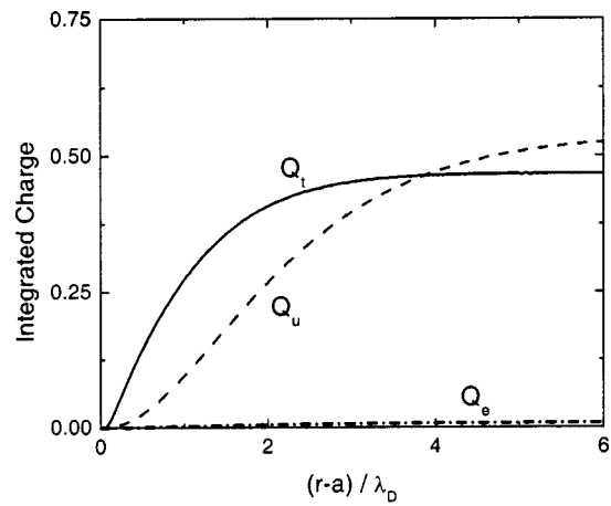
FIG. 3. Integrated trapped ion charge from r = a to r [ Q_t(r) , solid], deviation of the integrated untrapped ion charge from ambient [ Q_u(r) , dashed], and deviation of the integrated electron charge from ambient [ Q_e(r) , dotted–dashed], all scaled to the charge on the grain, for Case 1.
