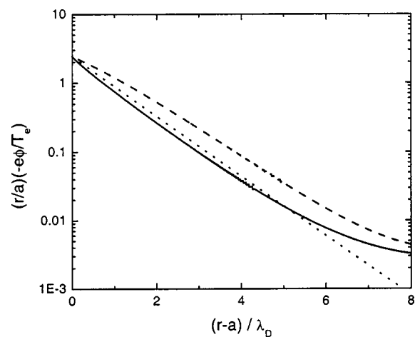
FIG. 4. Plot of -(r/a)e\phi(r)/T_e for Case 1: self-consistent potential including trapped ions (solid), potential with trapped ions neglected (dashed), Debye potential (dotted).
