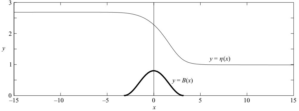
FIGURE 3. Computed hydraulic fall past a single submerged obstacle ( A_1=0 ) in the shape of the square of a cosine. The obstacle is characterized by A_2=0.4 and L_2=3.2 . The Froude number is found as part of the solution: F=1.977 .
