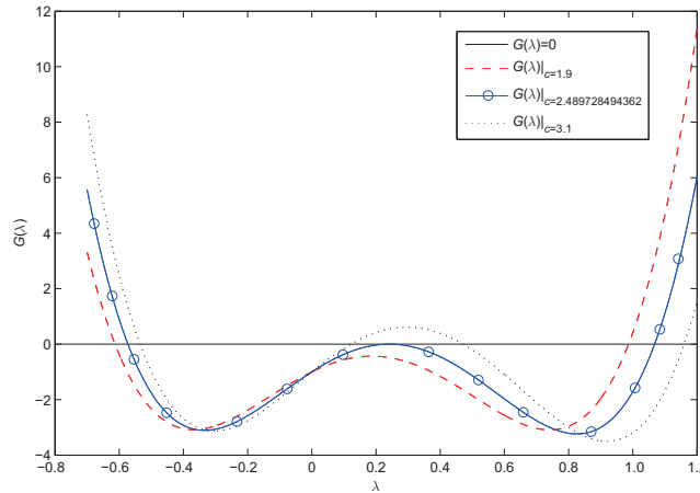
Figure 1 The curves of G(\lambda) when c takes different values. Let \alpha = 1 , \beta = 3 , \gamma = 2 , d_2 = 4 and d_3 = 7 be fixed. We can see that if c = c^* = 2.489728494362 , G(\lambda) has two simple real roots and a double real root; if c = 1.9 < c^* , G(\lambda) has two real roots; if c = 3.1 > c^* , G(\lambda) has four real roots
