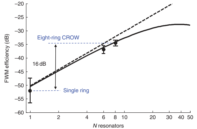
Figure 4 | Conversion efficiency versus the number of resonators. Marks indicate the measured conversion efficiency in a single resonator ( N=1 ) and in CROWs with 6 and 8 coupled resonators when P_p=12 dBm. All the structures have \text{FSR}=450 GHz and B=80 GHz. The higher error bar in the measurement of the single ring is due to the extremely low conversion efficiency ( < -50 dB), which is much lower than that of the 5-mm-long bus waveguide (about -36 dB). The dashed curve shows the theoretical conversion efficiency in absence of propagation loss in the CROW, whereas the solid curve takes into account 0.15 dB round trip loss in each ring of the CROW.
