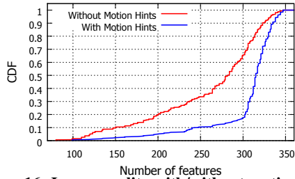
Figure 16: Image quality with/without motion hints.
