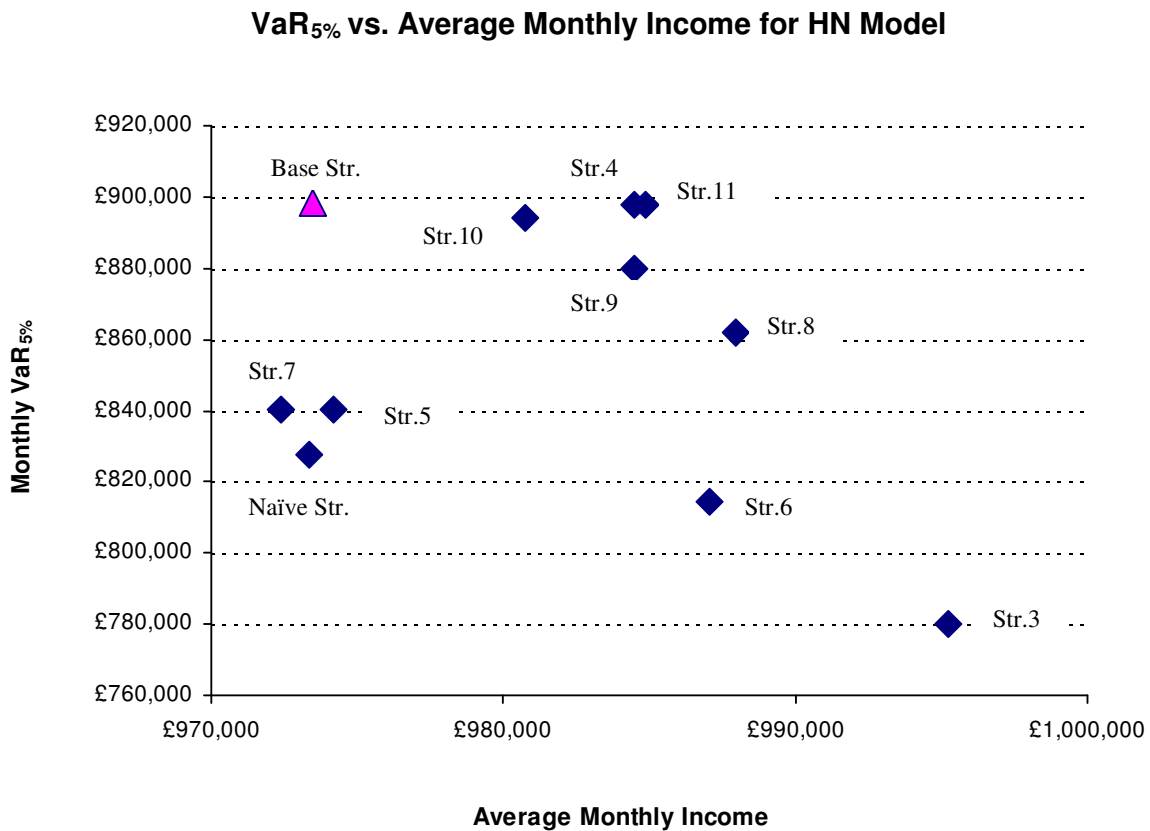
Figure 4-4 VaR 5% - Income relationship for HN model
