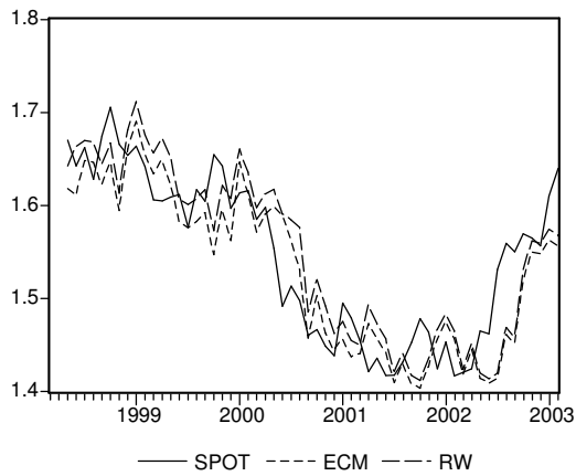
Figure 2-1 Random Walk vs. Error Correction Model out-of-sample forecasts comparison
