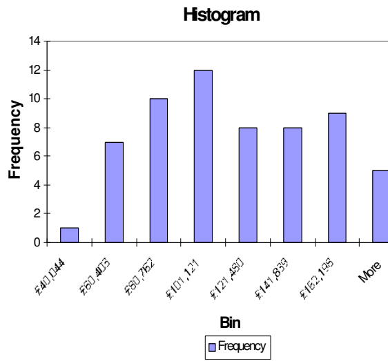
Figure 4-6 Histogram of EVPI for strategy 3
