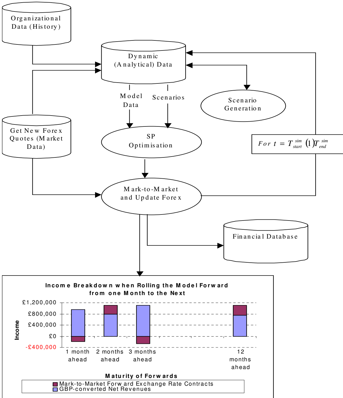
Figure 4-2 Rolling the model forward and “Mark to Market” process
