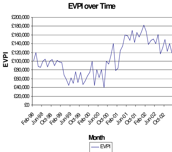
Figure 4-5 EVPI over time for strategy 3
