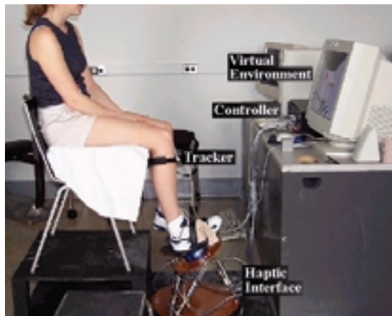
5 The Rutgers Ankle System. 39
