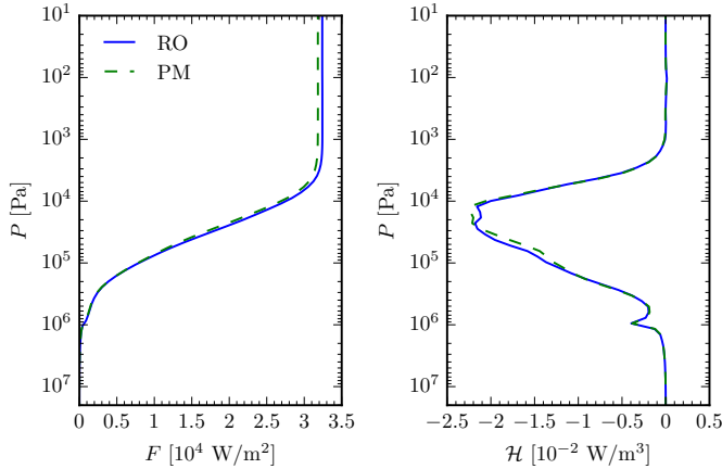
Fig. 10. Fluxes ( left ) and heating rates ( right ) obtained with the night side P - T profile in Fig. 3 using constant mixing ratios equal to the mixing ratios at P = 10^4 Pa, T = 1000 K. This eliminates errors caused by the implicit interpolation of mixing ratios with PM which dominates the errors seen using this overlap method in Figs. 8 and 9.
