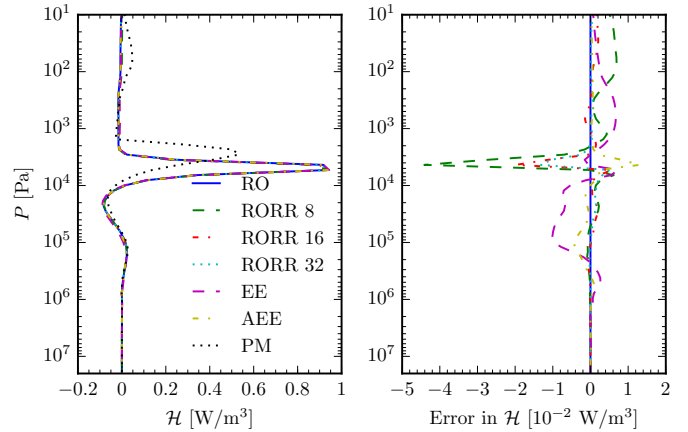
Fig. 12. Same as Fig. 11 but for heating rates. L1 norms of the errors (see the caption of Fig. 9) are 7.6% for RORR with n_k^{\text{bin}} = 8 , 3.0% for RORR with n_k^{\text{bin}} = 16 , 1.8% for RORR with n_k^{\text{bin}} = 32 , 7.0% for EE, 2.2% for AEE and 119% for PM.
