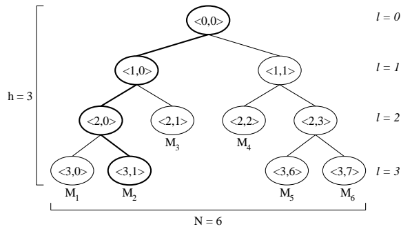
Fig. 1. Notation of a key tree
