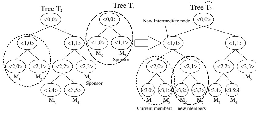
Fig. 9. Tree update in merge
