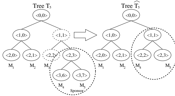
Fig. 5. Tree updating in leave operation
