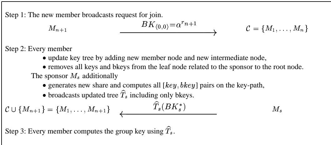
Fig. 2. Join Protocol
