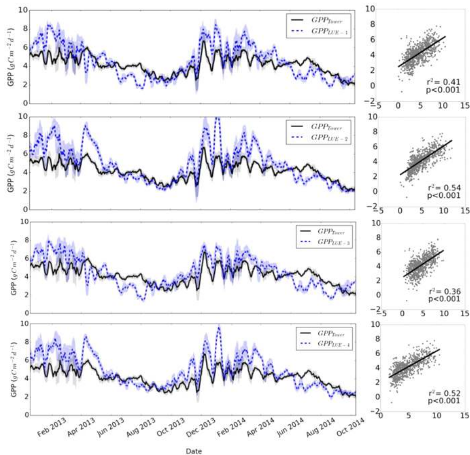
Figure 8. Overstorey flux tower estimated GPP with model predicted GPP for the Howard Springs OzFlux site. Models shown are (a) light use efficiency (LUE-1), (b) LUE with evaporative fraction (LUE-2), (c) LUE with green chromatic coordinates (LUE-3) and (d) LUE with EF and GCC (LUE-4).
