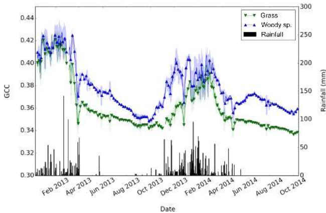
Figure 5. Daily rainfall (mm) and green chromatic coordinate (GCC) time series for grass and other woody green species (woody sp.) found in the savanna understory at the Howard Springs OzFlux site from December 2012 to October 2014. The GCC daily data are shown with an 8-day centred running mean (marked every 8 days for visualisation) applied. The standard error of the mean is given by the shading. The GCC time series represent the change in relative greenness of grass and woody species, not the absolute sum of grass versus woody species biomass in the understory.
