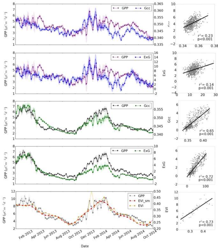
Figure 7. Overstory (a, b) and understory (c, d) flux tower GPP with green chromatic coordinate (GCC) and excess green (ExG) indices, as well as ecosystem flux tower GPP with MODIS enhanced vegetation index (EVI, e), from December 2012 to October 2014 at the Howard Springs OzFlux site. Daily data are shown with an 8-day running mean (marked every 8 days for visualisation) applied. The standard error of the mean is given by the shading. Included for each time series are the respective regression plots showing r^2 and p values for GCC–ExG–EVI ( x ) against flux tower GPP ( y ). For MODIS EVI (e) the time series plot includes raw 16-day values (EVI) and a Savitzky–Golay smoothed daily EVI product (EVI_sm), with the regression plot showing the raw 16-day EVI and the corresponding GPP for that day.
