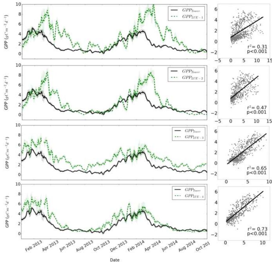
Figure 9. Understory flux tower estimated GPP with model predicted GPP for the Howard Springs OzFlux site. Models shown are (a) light use efficiency (LUE-1), (b) LUE with evaporative fraction (LUE-2), (c) LUE with green chromatic coordinates (LUE-3) and (d) LUE with EF and GCC (LUE-4).
