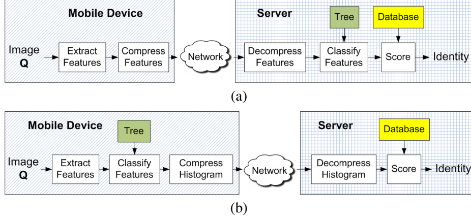
Figure 1. (a) Retrieval pipeline for compressing features and then classifying them at the server. (b) Retrieval pipeline for classifying features on the mobile device and then compressing the tree histogram.
