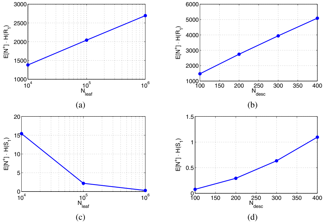
Figure 6. Joint entropy in bits for (a) R symbols versus N_{\text{leaf}} , for N_{\text{desc}} = 220 , (b) R symbols versus N_{\text{desc}} , for N_{\text{leaf}} = 10^6 , (c) S symbols versus N_{\text{leaf}} , for N_{\text{desc}} = 220 , and (d) S symbols versus N_{\text{desc}} , for N_{\text{leaf}} = 10^6 . Statistics reported for ZuBuD images.
