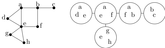
Figure 1: A graph with a tree decomposition
