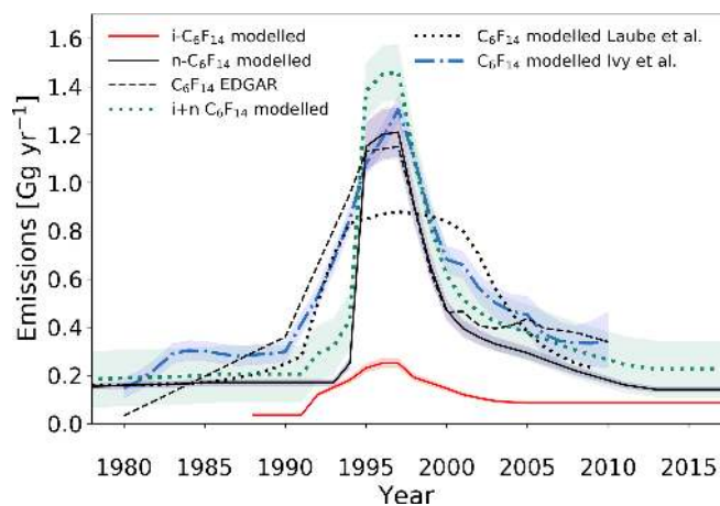
Figure 9. Estimated global emission rates for i\text{-C}_6\text{F}_{14} and n\text{-C}_6\text{F}_{14} in this study (full red and black lines, respectively) and global emission rates for \text{C}_6\text{F}_{14} as reported in the EDGARv4.2 database (dashed black line; no distinction between isomers), by Ivy et al. (2012b) (dash-dotted blue line; no distinction between isomers) and by Laube et al. (2012) (dotted black line; no distinction between isomers). The sum of the global emissions for the isomers of \text{C}_6\text{F}_{14} , as reported in the current work, is illustrated by the dotted green line. Shadings illustrate uncertainties.
