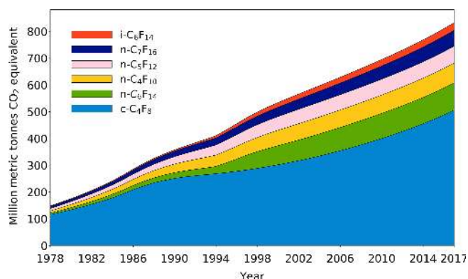
Figure 11. Cumulative CO 2 equivalent (million metric tonnes) of c-C 4 F 8 , n-C 4 F 10 , n-C 5 F 12 , i-C 6 F 14 , n-C 6 F 14 , and n-C 7 F 16 based on emissions between 1978 and 2017.
