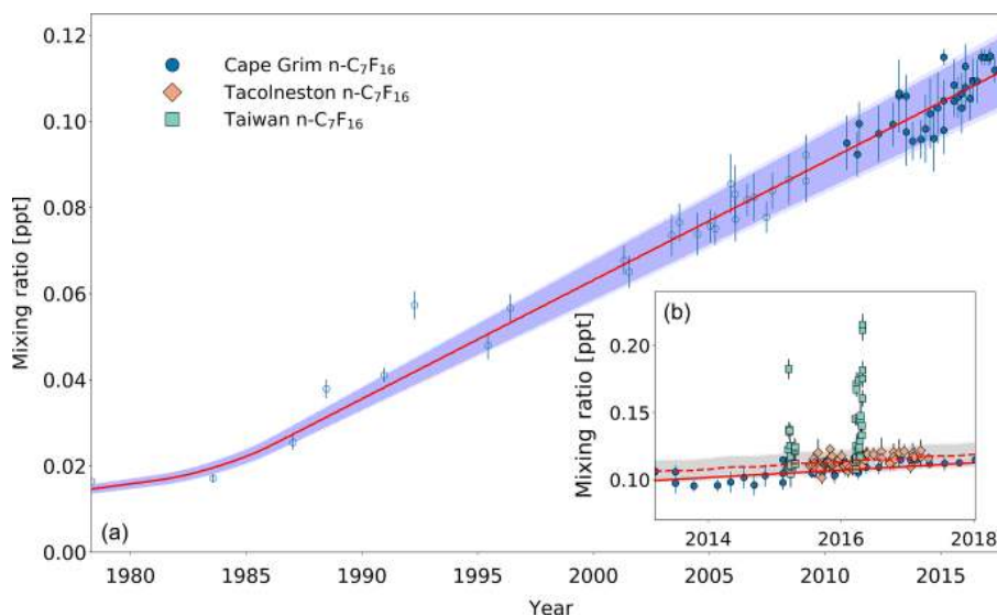
Figure 6. (a) Mixing ratios at Cape Grim of n\text{-C}_7\text{F}_{16} between 1978 and 2018 (blue circles). Data prior to 2010 are shown as empty markers, while data from samples collected after 2010 are shown as filled markers to illustrate the part of the time series that is extended in the current work. Note that the data from Laube et al. (2012) have been converted to a new and improved calibration scale. The atmospheric trend simulated by the model is represented by the red line. Total uncertainties (light blue) and trend uncertainties (dark blue) are indicated with the shaded areas along the trend line. (b) Mixing ratios after 2010 for Cape Grim (circles), for Tacolneston (diamonds), and Taiwan (squares). The red line indicates the modelled Southern Hemisphere baseline trend at Cape Grim, while the dashed red line indicates the modelled trend for mixing ratios at Tacolneston. Total and trend uncertainties are indicated with the shaded grey areas along the Tacolneston dashed-trend line.
