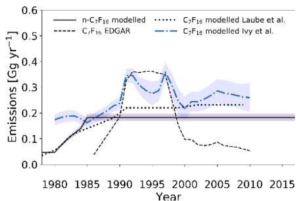
Figure 10. Estimated global emission rates for n\text{-C}_7\text{F}_{16} in this study (full black line) and global emission rates for \text{C}_7\text{F}_{16} as reported in the EDGARv4.2 database (dashed black line; no distinction between isomers), as reported in Ivy et al. (2012b) (dash-dotted blue line; no distinction between isomers) and as reported in Laube et al. (2012) (dotted black line; no distinction between isomers).
