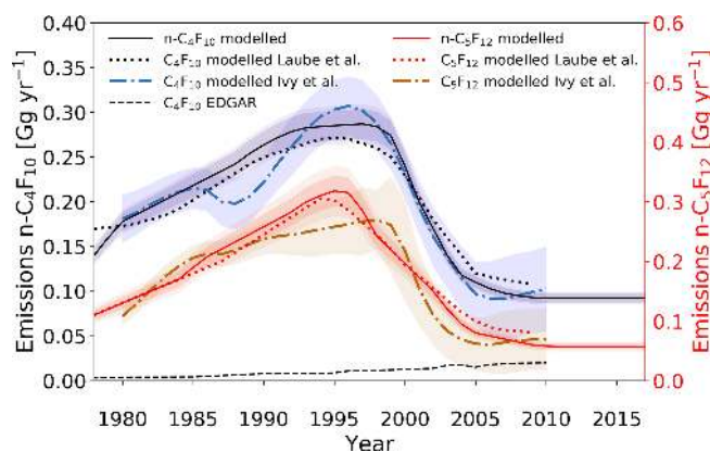
Figure 8. Estimated global emission rates for n-C 4 F 10 and n-C 5 F 12 (full black and red lines, respectively) in this study, global emission rates for C 4 F 10 as reported in the EDGARv4.2 database (dashed black line; no distinction between isomers), modelled emissions by Ivy et al. (2012b) for C 4 F 10 and C 5 F 12 (dash-dotted blue and brown lines, respectively; no distinction between isomers), and modelled emissions by Laube et al. (2012) for C 4 F 10 and C 5 F 12 (dotted black and red lines, respectively; no distinction between isomers). Note that the maximum EDGARv4.2 emission rate for n-C 5 F 12 is less than 0.6 \times 10^{-4} and is therefore not plotted here. Shadings illustrate the uncertainties.
