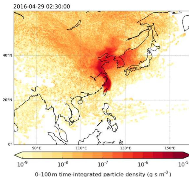
Figure 1. Example of the particle footprints generated by the NAME model indicating where air sampled in Taiwan came from. The colour scale is logarithmic and represents the calculated time-integrated particle density ( \text{g s m}^{-3} ) within the surface layer (0–100 m) during 12 d prior to the sampling days given a point release at Taiwan of \text{g s}^{-1} . Darker colours indicate a greater influence of the region on the chemical composition of the air sampled in Taiwan compared to the lighter colours.
