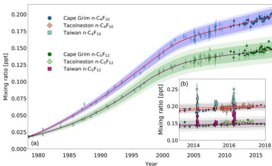
Figure 4. (a) Mixing ratios at Cape Grim of n-C 4 F 10 (blue circles) and n-C 5 F 12 (green circles) between 1978 and 2018. Data prior to 2010 are shown as empty symbols (Laube et al., 2012), while data from samples collected after 2010 are shown as filled symbols to illustrate the part of the time series that is extended in the current work. Note that the data from Laube et al. (2012) have been converted to a new and improved calibration scale. The atmospheric trends simulated by the model are represented by the red line for n-C 4 F 10 and by the magenta line for n-C 5 F 12 . Total uncertainties (light blue for n-C 4 F 10 , light green for n-C 5 F 12 ) and trend uncertainties (dark blue for n-C 4 F 10 , dark green for n-C 5 F 12 ) are indicated with the shaded areas along the trend line. (b) n-C 4 F 10 mixing ratios after 2010 for Cape Grim (blue circles), for Tacolneston (orange diamonds), and Taiwan (light blue squares); n-C 5 F 12 mixing ratios after 2010 for Cape Grim (green circles), for Tacolneston (light green diamonds), and Taiwan (magenta squares). The red and magenta lines indicate the modelled Southern Hemisphere baseline trend at Cape Grim for n-C 4 F 10 and n-C 5 F 12 , respectively, while the dashed red and magenta lines indicate the modelled trend for mixing ratios at Tacolneston for n-C 4 F 10 and n-C 5 F 12 , respectively. Total and trend uncertainties are indicated with the shaded grey areas along the Tacolneston dashed-trend lines for both n-C 4 F 10 and n-C 5 F 12 .
