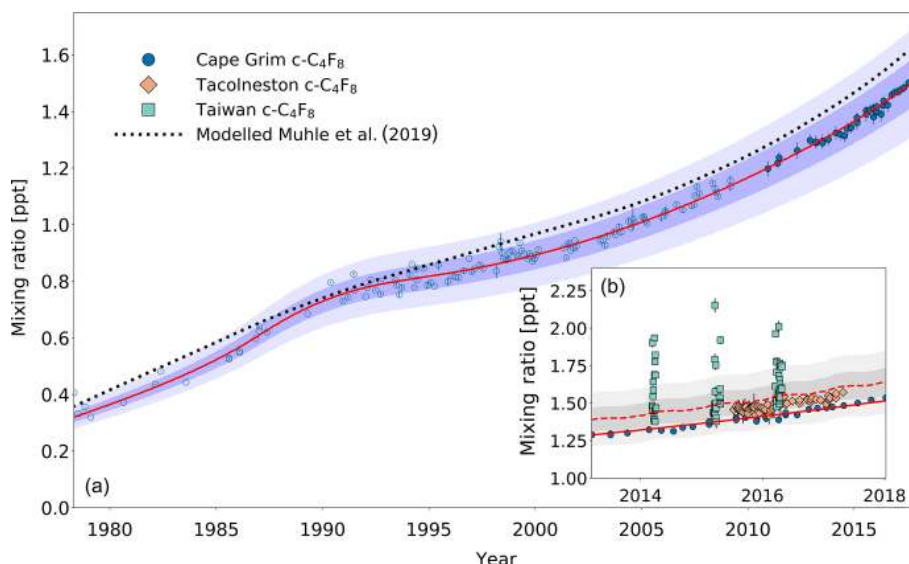
Figure 3. (a) Mixing ratios at Cape Grim of c\text{-C}_4\text{F}_8 between 1978 and 2018 (blue circles). Data prior to 2010 are shown as empty markers (Oram et al., 2012), while data from samples collected after 2010 are shown as filled markers to illustrate the part of the time series that is extended in the current work. The atmospheric trend simulated by the model is represented by the red line. Total uncertainties (light blue) and trend uncertainties (dark blue) are indicated with the shaded areas along the trend line. Results for the c\text{-C}_4\text{F}_8 trend published in Mühle et al. (2019) are shown in the dotted black line. (b) Mixing ratios after 2010 for Cape Grim (circles), for Tacolneston (diamonds), and Taiwan (squares). The red line indicates the modelled Southern Hemisphere baseline trend at Cape Grim, while the dashed red line indicates the modelled trend for mixing ratios at Tacolneston. Total and trend uncertainties are indicated with the shaded grey areas along the Tacolneston dashed-trend line.
