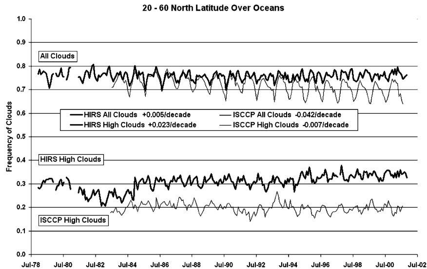
FIG. 5. The monthly average frequency of clouds from 20^{\circ} to 60^{\circ} N over oceans.
