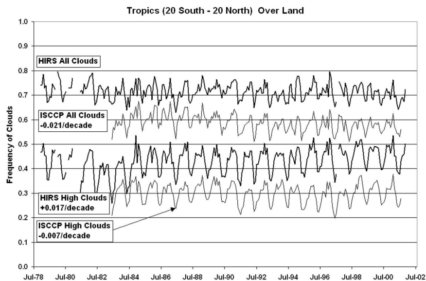
FIG. 6. The monthly average frequency of clouds from 20^{\circ} S to 20^{\circ} N over land.
