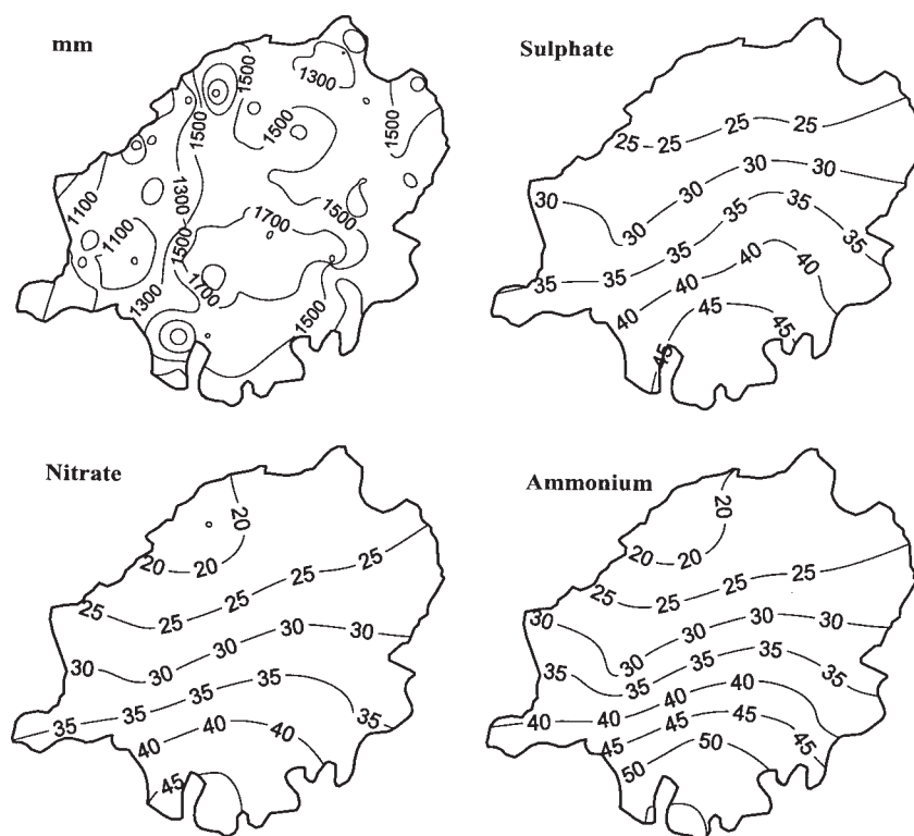
Fig. 2. Distribution map of the amount of precipitation and of the concentrations of \text{SO}_4 , \text{NO}_3 and \text{NH}_4 (meq \text{l}^{-1} ) in wet deposition in the Lake Maggiore catchment in 1997
