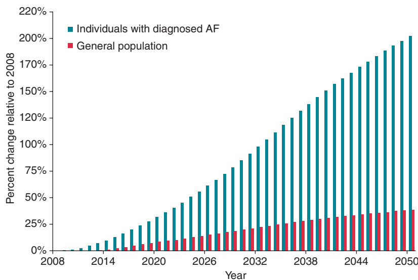
Figure 3 Estimated percentage changes in the number of individuals 20–99 years of age with AF in Iceland assuming a continued increase in incidence as evident in 1991–2008 and mortality according to projections for Iceland, and the Icelandic population 20–99 years of age relative to 2008 values.
