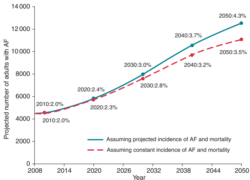
Figure 2 Projected burden of diagnosed AF in 20–99 year olds in Iceland 2008–2050 assuming no change in the incidence of AF and mortality beyond 2008 and assuming a continued increase in incidence as evident in 1991–2008 and mortality according to projections for Iceland. Data labels present prevalence figures in selected years.
