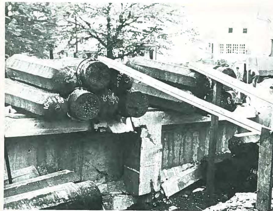
Fig. 18a. Closeup of failure at midspan.
