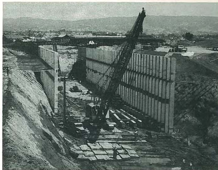
Fig. 54. Contractor's graving dock for manufacture of sub-aqueous vehicular tubes at Webster Street Tube, Oakland-Alameda, California, 1960. Pretensioned concrete soldier beams are designed for maximum negative moments through the addition of mild steel.
