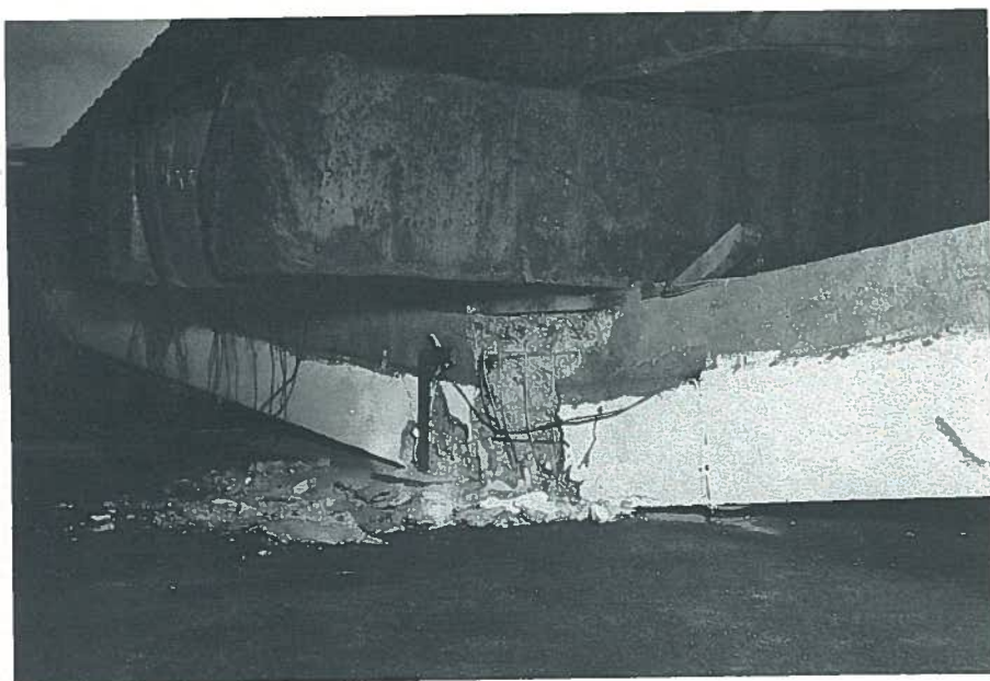
Fig. 23. Closeup of fracture. Note wires leading to strain gages on beam. (Pottstown prototype girder.)
