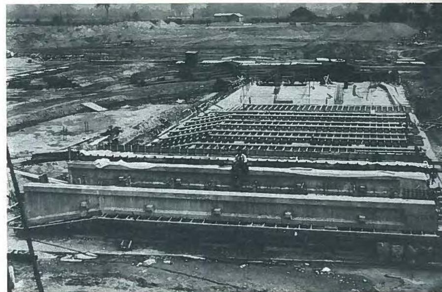
Fig. 2. Post-tensioned beams for the Canadian Army Ordnance Warehouse at Cobourg, Ontario, 1952 (Magnet system).
