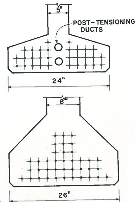
Fig. 72. Top drawing shows that by using post-tensioning tendons and re-arranging the strand, a more efficient section (with a better utilization of prestressing) results as compared to the bulkier AASHTO section shown below.
