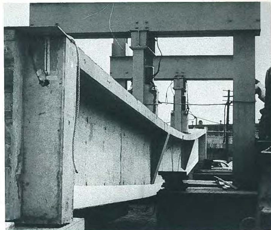
Fig. 38. Loading of 60-ft (18.3 m) prestressed girder (F-60) using bonded tendons. At four times the design load the girder deflected 12 in. (305 mm), displaying enormous ductility and prompting a reporter to headline "Rubber Concrete Carries Severe Overload."
