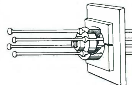
Fig. 17. Double-headed wire with anchorage.
