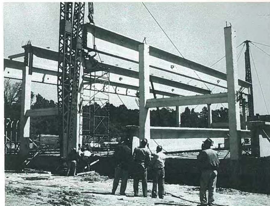
Fig. 40. Girder No. 3 almost in position over columns. The column cables are being pulled up in order to thread them through holes in the girder ends.
