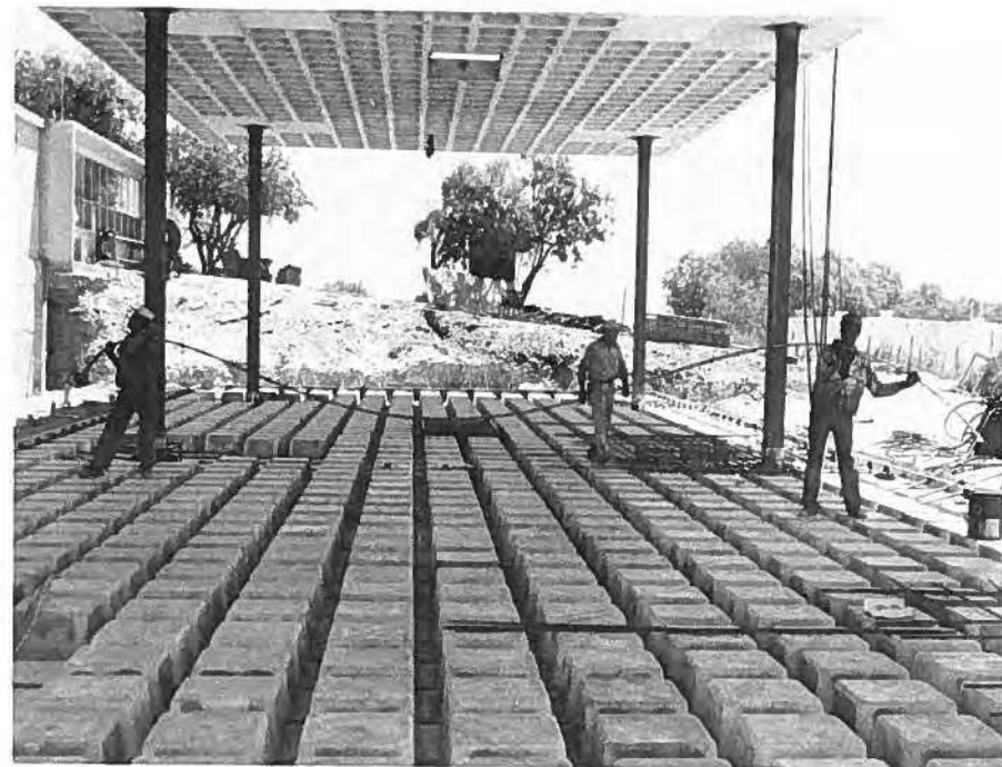
Fig. 18. Prestressing tendons being placed in waffle slab (Southwest Research Institute, San Antonio, Texas).
