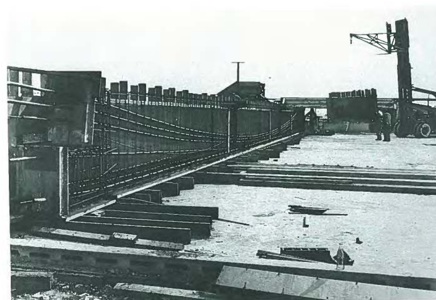
Fig. 76. Formwork for Klickitat County bridge girder showing rubber extractable cores and reinforcing in place prior to casting. Note dividers to separate beam into three segments.
