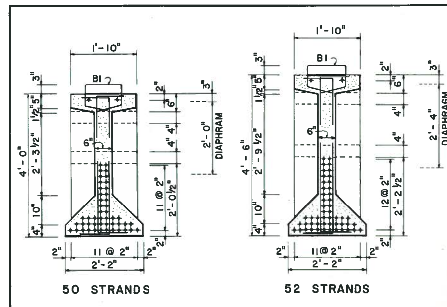
Fig. 29. At left, the BPR's proposed 70-ft span pretensioned standard girder for 24-ft roadway and H15-44 loading. At right, the proposed 70-ft span pretensioned standard girder for 28-ft roadway and H20-S16-44 loading. Their unwarranted difficulty in manufacture should be evident.
