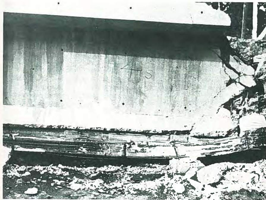
Fig. 18b. Closeup of failure due to moments.
