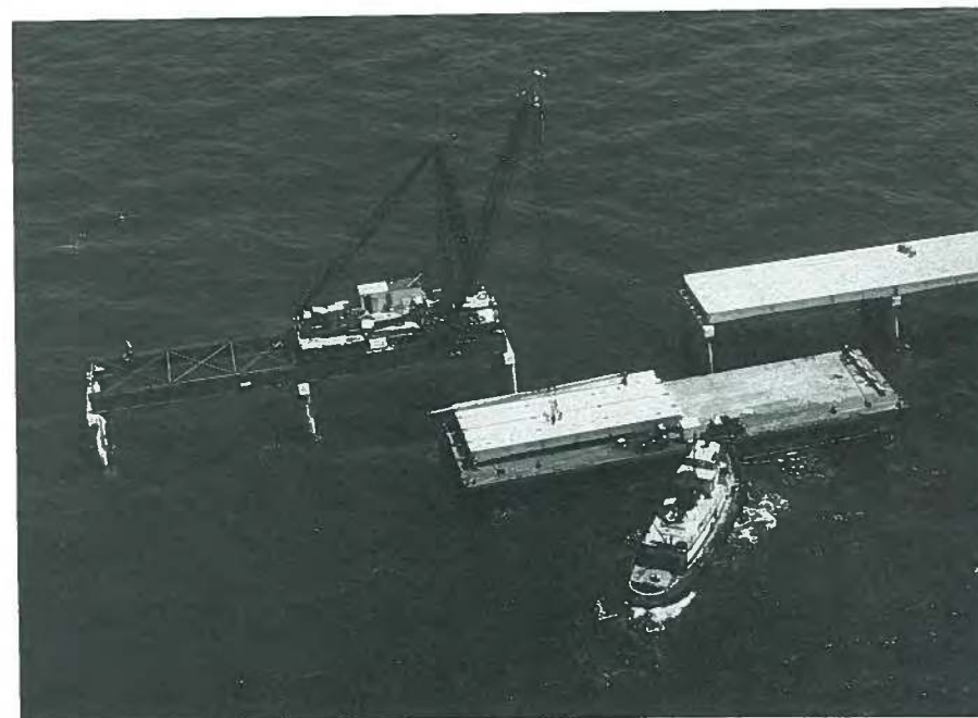
Fig. 7. General view of erection of a span to be part of the Chesapeake Bridge-Tunnel Crossing connecting Cape Charles to Norfolk, Virginia.
