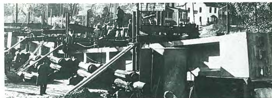
(c) Girder after failure.
