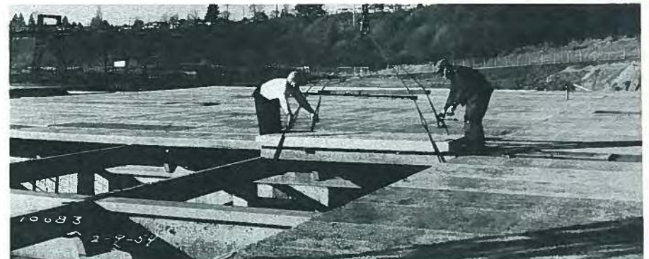
Fig. 65. Lightweight roof slabs are lowered, two at a time, into place across the structural frame. The precast slabs are 40 in. (1.02 m) wide, 10 ft (3.05 m) long and 1½ in. (38.1 mm) thick, with a 6-in. (152 mm) leg.
