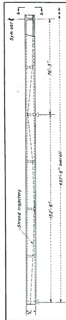
ELEVATION of a three-span box girder shows the strands placed high in the cells over the piers, low near midspan to vary the prestress.
