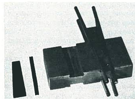
Fig. 1. Magnel "wedge" and Freyssinet "cone" friction anchorages.
