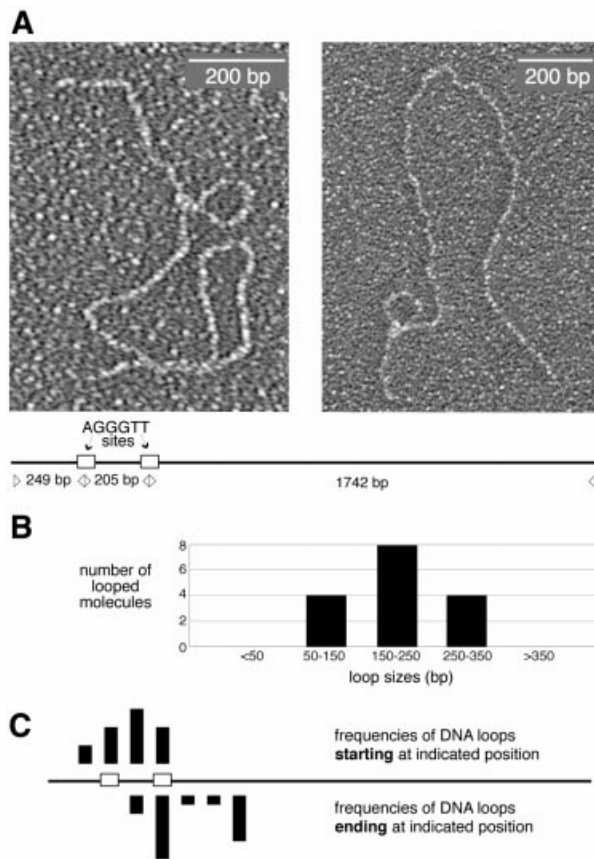
Fig. 5. EM analysis of TRF1-inducing loops between two half-sites separated by 205 bp. (A) Electron micrographs of linear DNA molecules containing two AGGGTT sites bearing small DNA loops anchored at their base by a TRF1 protein ball. Schematic of the DNA fragment [ NaeI – ScaI fragment from pBluescript II KS(+)] is shown below the micrographs. (B) Histogram of the TRF1-induced loop sizes on the NaeI – ScaI fragment. (C) Histogram of the positions of bound TRF1 molecules in the NaeI – ScaI fragment.
