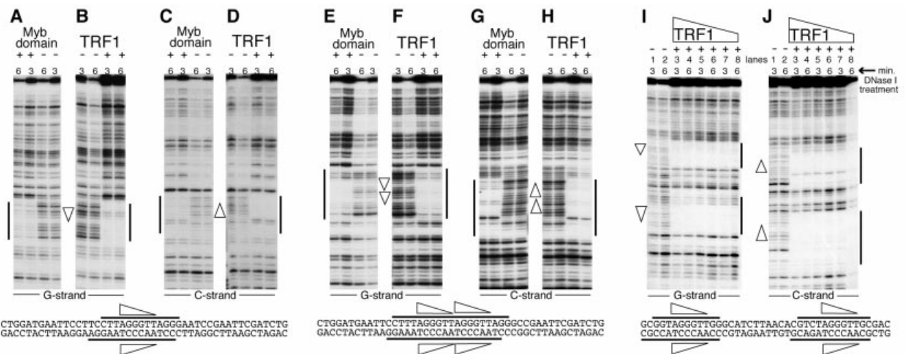
Fig. 4. Footprinting of TRF1 and the isolated Myb domain on DNA fragments containing one or two copies of the half-site. (A–D) DNase I footprint of the isolated TRF1 Myb domain and dimeric TRF1 bound to a single half-site. (E–H) DNase I footprint of the Myb domain and TRF1 bound to two adjacent half-sites. (I and J) DNase I footprint of dimeric TRF1 bound to two non-adjacent half-sites. Protected positions were assessed from G+A Maxam–Gilbert sequencing reactions run in parallel (not shown). Open triangles indicate the 5'-AGGGTT-3' core sequence. Bars highlight protected regions. The TRF1 concentration was 2 \times 10^{-8} M for (B), (D), (F) and (H), and reactions were performed with 10 \mu\text{g/ml} sonicated calf thymus competitor DNA. For (I) and (J), TRF1 concentrations were 2 \times 10^{-8} M (lanes 3 and 4), 6 \times 10^{-9} M (lanes 5 and 6) and 2 \times 10^{-9} M (lanes 7 and 8), and sonicated E. coli DNA was used as a competitor.
