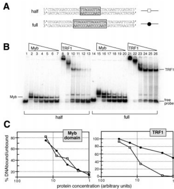
Fig. 2. Band-shift analysis of binding of TRF1 and the Myb domain to DNA fragments containing one or two copies of the half-site. (A) DNA probes used in binding assays. DNAs 'half' and 'full' were restriction fragments of 111 and 117 bp, respectively, containing the telomeric sequences indicated. (B) Band-shift assay for TRF1 and the TRF1 Myb domain binding to the 'half' and 'full' DNA probes. Assays were performed under standard TRF1 conditions with addition of 0.1% NP-40 and poly(dI-dC) (100 ng). Gel was run in 0.5× TBE at 4°C. Protein concentrations varied in 2-fold serial dilutions starting from \sim 4 \times 10^{-7} M for TRF1 and \sim 1.0 \times 10^{-7} M for the Myb domain. (C) Phosphorimager quantitation of reactions shown in (A). All complexes were scored as protein-bound DNA (both complexes in the case of the Myb domain).
