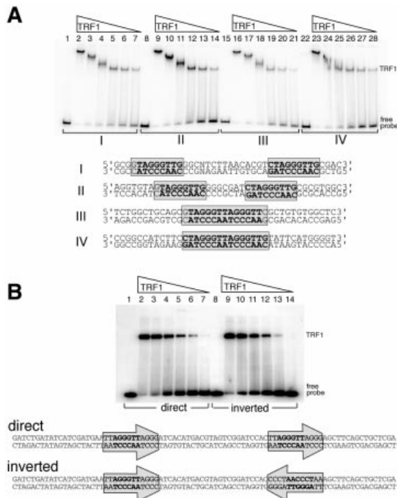
Fig. 3. Effects of spacing and orientation of half-sites on TRF1 binding. (A) TRF1 band-shift assays on four representative clones recovered from SELEX, two from each class of sites. DNA probes were 170 bp, with the TRF1 half-sites (boxed) at a central position. Within each box, matches to the consensus are indicated in bold. The protein concentrations were a dilution range with 1.5-fold steps starting at \sim 1.7 \times 10^{-7} M (lanes 2, 9, 16 and 23). The position of the unbound DNA and the TRF1–DNA complex are indicated at the right of the gel. (B) TRF1 band-shift assays on two DNA fragments bearing two half-sites in either direct or inverted orientation. Protein concentrations varied in 2-fold steps beginning at about 1.4 \times 10^{-7} M (lanes 2 and 9). The size of the DNA fragments was 80 bp. Telomeric cassettes are highlighted on gray background, and core sites are in bold.
