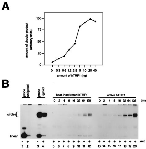
Fig. 6. hTRF1 enhances DNA cyclization. (A) Effect of increasing amounts of baculovirus-expressed hTRF1 on cyclization of a 217 bp DNA fragment containing 27 TTAGGG repeats. (B) The rate of cyclization of the 217 bp DNA fragment was measured in the presence of either heat-inactivated (lanes 5–12) or active (lanes 13–20) baculovirus-expressed hTRF1. Ligation time (in minutes) is indicated over lanes 5–20. Exonuclease digestion was performed as indicated prior to loading of samples in order to eliminate linear ligation products. Lanes 1 and 2 show unligated samples. In lanes 3 and 4, the fragment was ligated with a 20-fold higher concentration of ligase as compared with samples 5–20. Lane 4 is under-loaded due to loss of DNA after exonuclease digestion.
