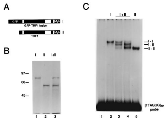
Fig. 2. hTRF1 binds DNA as a dimer. (A) Schematic representation of the two hTRF1 derivatives (I and II) that differed in size by ~26 kDa. Form I contains the 26 kDa GFP protein fused to the N-terminus of hTRF1. Form II contains an N-terminal addition of 43 amino acids encoded by polylinker sequences. (B) SDS-PAGE gel showing [ 35 S]methionine-labeled products resulting from in vitro translation of the hTRF1 derivatives depicted in (A). (C) Gel-shift assay with hTRF1 derivative I (lane 2), hTRF1 derivative II (lane 5) or a mixture of the two (lanes 3 and 4). The probe is a restriction fragment containing the sequence [TTAGGG] 12 . For the reactions in lanes 3 and 4, the hTRF1 derivatives were produced by co-translation. The ratio of plasmids used in the coupled transcription–translation reaction was 1:1 for lane 3 and 1:2 (excess of hTRF1 derivative II) for lane 4. Lane 1 represents a reaction with mock in vitro translation product. The protein compositions of the gel-shift complexes are indicated to the right of the gel.
