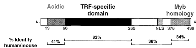
Fig. 1. Schematic of the domains of human TRF1 (hTRF1) and their conservation in mouse TRF1 (mTRF1) (adapted from Broccoli et al. , 1997).
