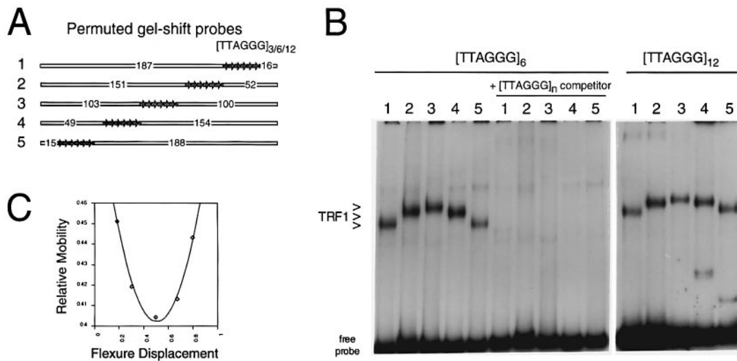
Fig. 5. hTRF1 bends DNA. (A) Schematic representation of two sets of five PCR-generated permuted gel-shift probes carrying either three, six or 12 complete tandem TTAGGG repeats. The length of the non-telomeric sequences in each of the probes is indicated. (B) Gel-shift assay with partially purified HeLa TRF1 and the labeled probes shown in (A). The assay on the left side was performed with probes containing [TTAGGG] 6 sites with or without added unlabeled [TTAGGG] n competitor DNA as indicated. The assay on the right hand side was performed with probes containing [TTAGGG] 12 sites. (C) Plot of the relative mobility (mobility of bound DNA/mobility of free DNA) of each of the TRF1 complexes against the flexure displacement in each probe. The data points represent probes 1–5 from right to left; values on the x-axis indicate the distance from the middle of the TTAGGG repeat site to the 5' end of the probe divided by the length of the probe. The data points were interpolated with the function derived by Ferrari et al. (1992).
