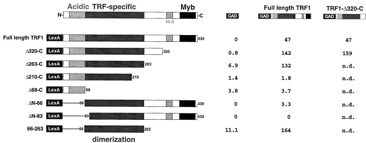
Fig. 3. Identification of the dimerization domain of hTRF1 using the two-hybrid system. \beta -Galactosidase levels were measured for strains containing plasmids expressing various LexA-TRF1 hybrid genes (as indicated) along with plasmids expressing either the GAL4 activation domain (GAD) or GAD fusions containing full-length or truncated ( \Delta 320-C) TRF1. The values represent an average of three independent transformants. Values <0.01 are indicated by 0; n.d. = not determined.
