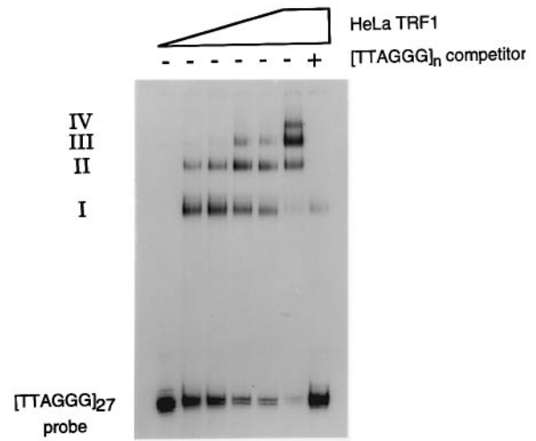
Fig. 7. hTRF1 dimers do not show strong cooperative interactions. Increasing amounts (1, 2, 3, 4 and 8 \mu l) of partially purified HeLa TRF1 was added to a labeled probe derived from plasmid pTH5 (de Lange et al. , 1990) which carries 27 tandem TTAGGG repeats. Complexes containing 1–4 TRF1 dimers are identified to the left of the gel (Roman numerals). The first lane is a mock reaction in the absence of hTRF1. Unlabeled TTAGGG repeat competitor DNA was added to the reaction in the last lane.
