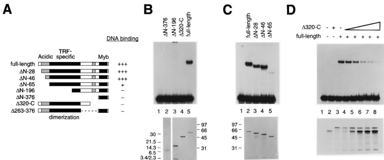
Fig. 4. Deletion mapping of the sequences in hTRF1 required for DNA binding. (A) Schematic of the deletion mutants used and summary of their DNA-binding activity. (B) and (C) Gel-shift reactions with the indicated hTRF1 derivatives. (D) Co-translation experiments showing that hTRF1 requires two Myb repeats for DNA binding. Increasing amounts of \Delta 320\text{-C} were co-translated with full-length hTRF1 and the mixtures were assayed for TTAGGG repeat-binding activity. The gel-shift probe in (B–D) is a [TTAGGG] 12 -containing restriction fragment. To ensure that each protein was present at the same concentration, the proteins were synthesized in parallel in the presence of [ 35 S]methionine and the labeled products were analyzed on SDS-PAGE (shown below each of the gel-shift assays).
