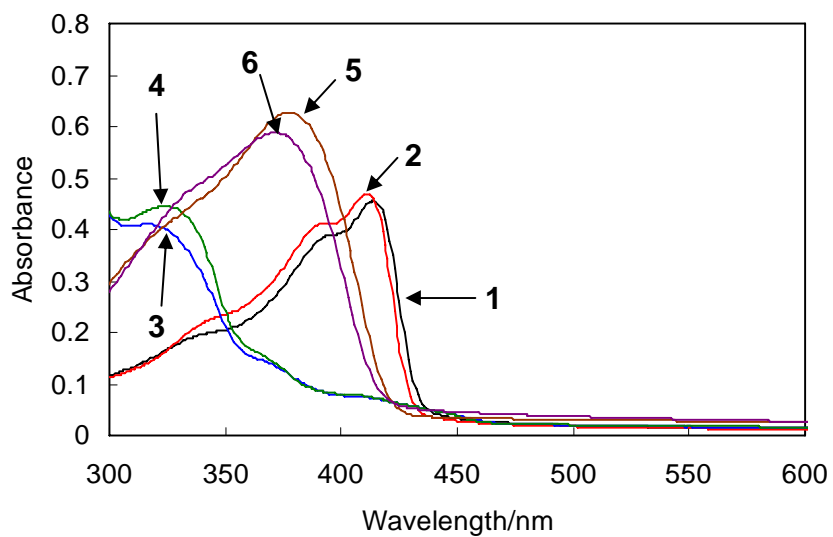
Supporting Figure 1. UV-vis spectra of 1 - 6 in film spin coated on glass from 1.5wt% of polymer solution in chlorobenzene.
