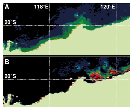
Fig. 5. (A) Image of chlorophyll and (B) relative Trichodesmium abundance derived from a coastal zone color scanner (CZCS) image of the northwestern coast of Australia in the vicinity of the Dampier Archipelago and confirmed by contemporaneous sea-truth data [adapted from (42)]. A protocol based on reflectivity and absorption at 550 nm was used. Chlorophyll is reported as detected by CZCS, with lowest to highest chlorophyll a concentrations ranging from purple (<0.05 \text{mg m}^{-3} ) to red (>3.0 \text{mg m}^{-3} ). For Trichodesmium , dark colors indicate its absence; lighter colors (light blue through orange) indicate its presence. Differences in color represent varying responses to the protocol, not necessarily differences in Trichodesmium concentration.
