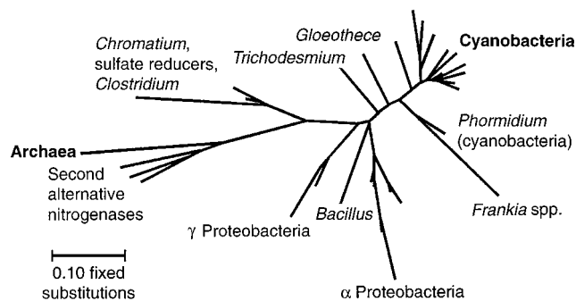
Fig. 3. Evolutionary relation of the genus Trichodesmium to other diazotrophs on the basis of nifH amino acid sequence data. The evolutionary distances between deduced amino acid sequences were used to create a phenogram using the neighbor-joining method of PHYLIP (96). The Fe protein gene ( nifH ) of Trichodesmium was amplified from cultures by means of the polymerase chain reaction
