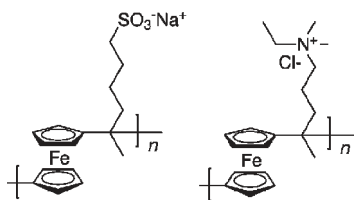
Figure 6. Ferrocene-containing polymers used for electrochemical triggering. 65
