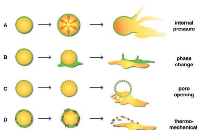
Figure 5. Physical methods of capsule release: (A) shell wall rupture by an increase in internal pressure, (B) melting of the polymer shell wall, (C) change in porosity of the shell wall resulting from a phase transition of a shell wall polymer, and (D) disintegration of the shell wall utilizing nanoparticles that oscillate in response to an external trigger.
