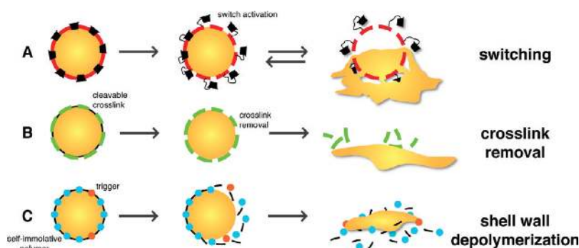
Figure 4. Methods for the chemical disassembly of microcapsule shell walls: (A) opening of pores in the shell wall by a switching mechanism, (B) chemical cleavage of incorporated cross-links resulting in decomposition of the shell wall, and (C) a self-immolative process in which triggers initiate depolymerization of the shell wall.
