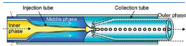
Figure 3. Schematic of a microcapillary device used for generating double emulsions. 55
