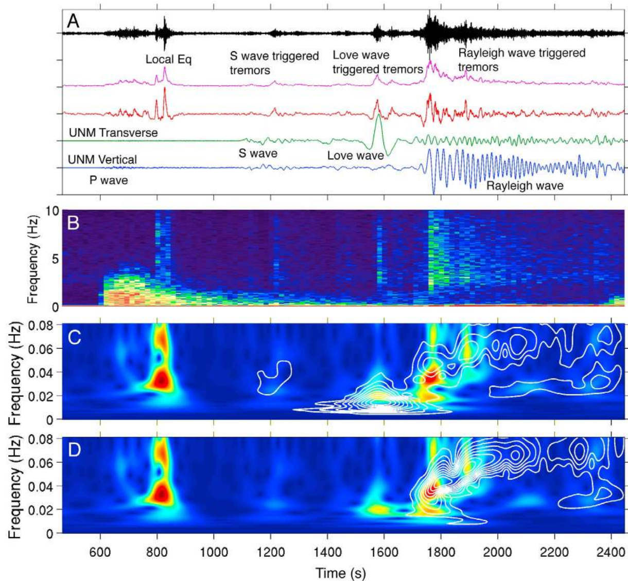
Figure 3. (a) Comparison between the 2–8 Hz filtered data recorded on a short period sensor at ATLI (black trace) and the broadband record of the Chilean earthquake at the UNM station in Mexico City for the transverse (green trace) and vertical (blue trace) components. The time scale is in seconds and starts at the initial time of the Maule earthquake. The envelope function of the ATLI data is in purple. The red trace is the high pass filtered envelope function that clearly shows the variations in the tremor activity. There is a clear triggering of tremor in ATLI by the S wave packet, the Love wave and the Rayleigh wave. A careful look at the envelope of this triggered tremor (Figure 3a, purple trace) shows a decrease of the seismic energy radiated by the NVT bursts and a temporal decrease of their duration. This observation reveals a dispersion in the envelope of the triggered tremor. (b) Spectrogram of the data recorded at ATLI. (c, d) We compare the S-transform spectrogram obtained for the high pass filtered envelope presented in Figure 3a (color plot) with the S-transform spectrograms obtained for the raw broadband records at UNM station (white contours). Figure 3c shows the transverse component, and Figure 3d shows the vertical component. The comparison of the dispersion observed in the envelope of tremors (color plot) with the one associated with Rayleigh waves recorded in Mexico City (Figure 3d) shows the modulation of the tremors by the dispersed waves.
