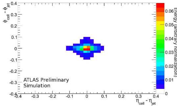
Figure 11: Energy distribution for jets that originate from \pi^0 's that decay inside of the barrel HCal, where (0,0) is the jet axis.
