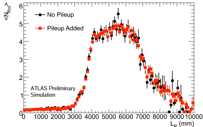
Figure 9: Average number of L1 muon RoIs vs \pi_\nu^0 decay distance.
