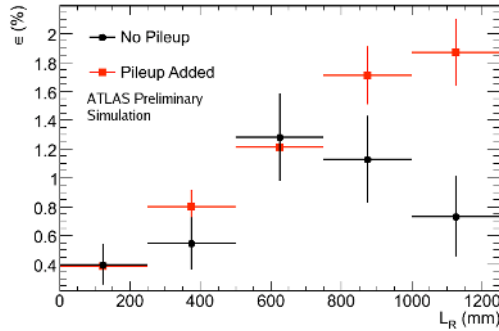
Figure 25: Efficiency for the Trackless Jet + muon trigger as a function of the \pi^0 decay position for decays in the barrel region.
