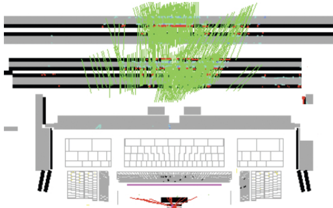
Figure 5: ATLANTIS display (longitudinal view) of a \pi^0 decay in the barrel muon spectrometer.
