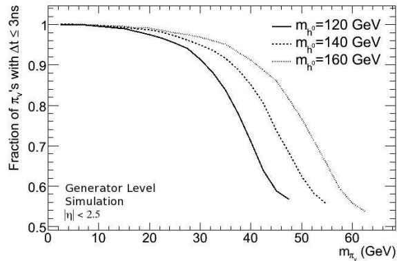
Figure 22: Fraction of \pi_v^0 's that decay in the HCal with a \Delta t shift < 3 ns as a function of the \pi_v^0 mass.
