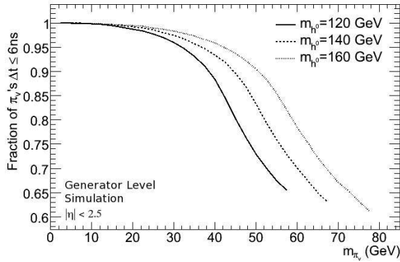
Figure 20: Fraction of \pi_\nu^0 's with a \Delta t shift < 6 ns as a function of the \pi_\nu^0 mass.
