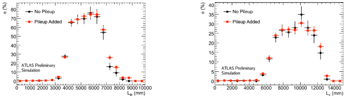
Figure 23: Efficiency for the muon RoI cluster trigger as a function of the \pi^0 decay position for decays in the barrel (Left) and endcap (Right).
